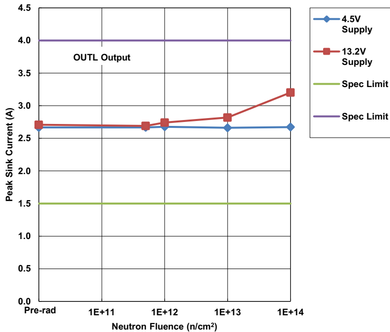
Figure 19. ISL70040SEH median OUTL peak sink current ( I_{SNK} ), C_L = 220\text{nF} , as a function of total dose irradiation at low and at high dose rate for the biased and as a function of neutron irradiation at 5 \times 10^{11} , 1 \times 10^{12} , 1 \times 10^{13} , and 1 \times 10^{14}\text{n/cm}^2 . The sample size of all four cells was five per cell. The SMD limits are 1.5A to 4.0A.
