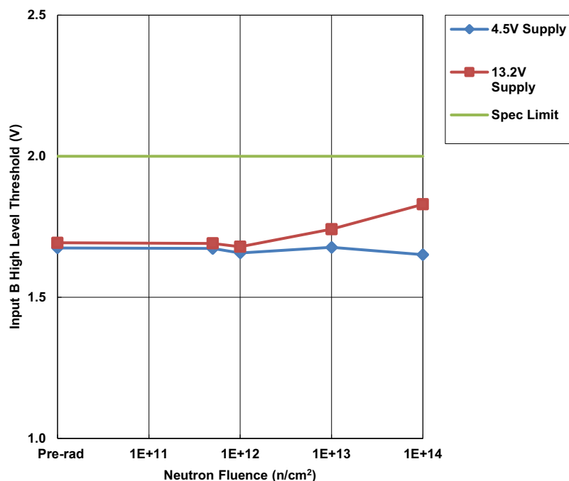
Figure 6. ISL70040SEH median input B HIGH level threshold ( V_{IH} ), 4.5V and 13.2V supply, as a function of neutron irradiation at 5 \times 10^{11} , 1 \times 10^{12} , 1 \times 10^{13} , and 1 \times 10^{14} n/cm 2 . The sample size of all four cells was five per cell. The SMD limit is 2.0V maximum (4.5V supply and 13.2V supply).
