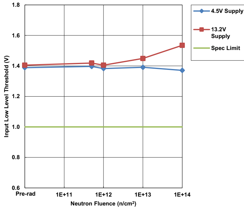
Figure 5. ISL70040SEH median input LOW level threshold ( V_{IL} ), 4.5V and 13.2V supply, as a function of neutron irradiation at 5 \times 10^{11} , 1 \times 10^{12} , 1 \times 10^{13} , and 1 \times 10^{14} n/cm 2 . The sample size of all four cells was five per cell. The SMD limit is 1.0V minimum (4.5V supply and 13.2V supply).
