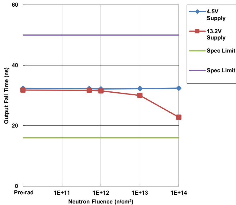
Figure 9. ISL70040SEH median fall time ( t_{\text{FALL}} ) as a function of total dose irradiation at low and at high dose rate, 10nF load capacitance, as a function of neutron irradiation at 5 \times 10^{11} , 1 \times 10^{12} , 1 \times 10^{13} , and 1 \times 10^{14} \text{ n/cm}^2 . The sample size of all four cells was five per cell. The SMD limits are 16ns to 50ns.
