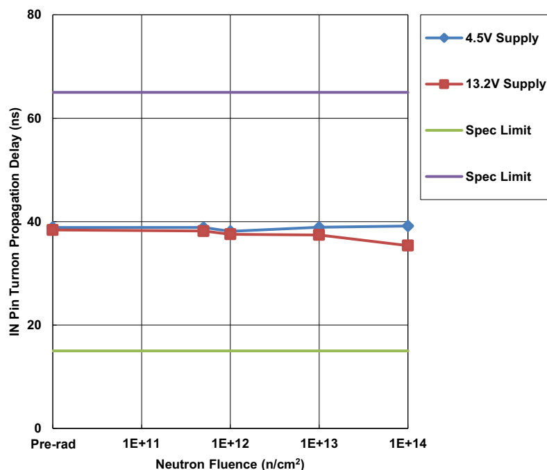
Figure 10. ISL70040SEH median input to output turn-on propagation delay ( t_{\text{DON}} ), 4.5V and 13.2V supply, as a function of neutron irradiation at 5 \times 10^{11} , 1 \times 10^{12} , 1 \times 10^{13} , and 1 \times 10^{14} \text{ n/cm}^2 . The sample size of all four cells was five per cell. The SMD limits are 15ns to 65ns.
