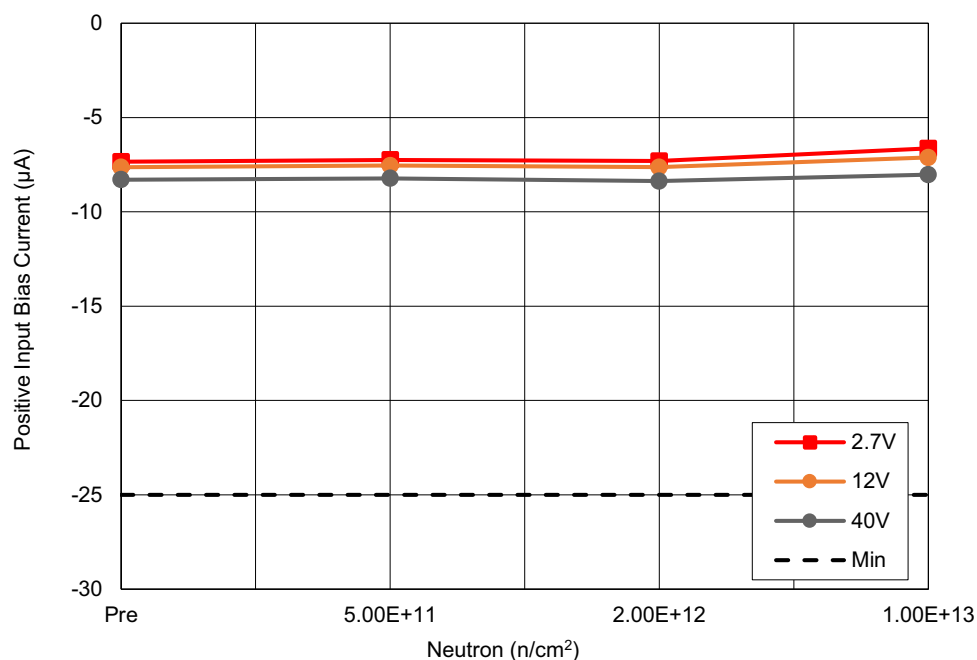
Figure 11. ISL7x100SEH positive input bias current ( I_{BIAS+} ) with V_+ = 2.7V , 12V and 40V , V_{RS+} = 0V , and V_{SEN} = 0mV , following irradiation to each level. The error bars (if visible) represent the minimum and maximum measured values. The post-irradiation SMD limit is -25\mu A minimum.
