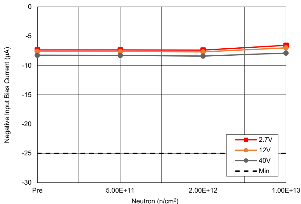
Figure 12. ISL7x100SEH negative input bias current ( I_{BIAS-} ) with V_+ = 2.7V , 12V and 40V , V_{RS+} = 0V , and V_{SEN} = 0mV , following irradiation to each level. The error bars (if visible) represent the minimum and maximum measured values. The post-irradiation SMD limit is -25\mu A minimum.
