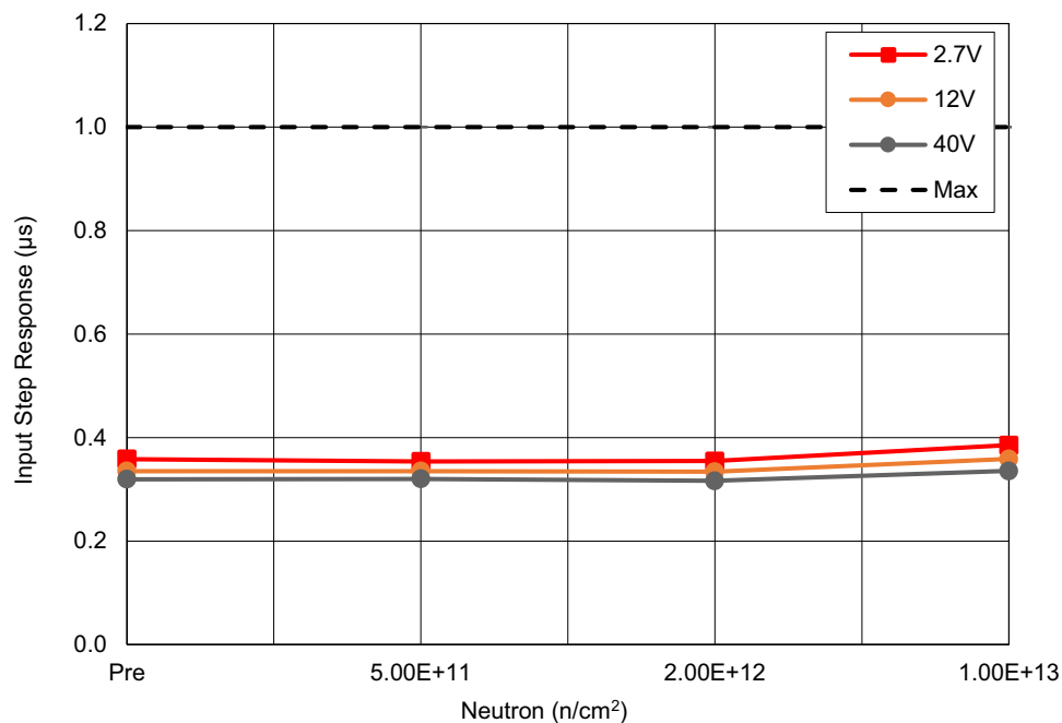
Figure 40. ISL7x100SEH input step response time ( t_{RES} ) with V^+ = 40V , 12V , and 2.7V , V_{SEN} = 5mV to 150mV , following irradiation to each level. The error bars (if visible) represent the minimum and maximum measured values. The post-irradiation SMD limit is 1\mu s maximum.
