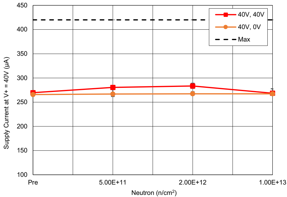
Figure 35. ISL7x100SEH supply current ( I_+ ) with V_+ = 40V , V_{SEN} = 0V , V_{RS+} = 40V and 0V , following irradiation to each level. The error bars (if visible) represent the minimum and maximum measured values. The post-irradiation SMD limit is 420\mu A maximum.
