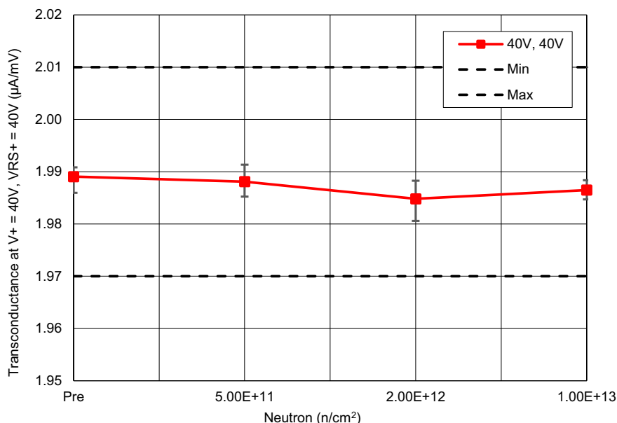
Figure 2. ISL7x100SEH transconductance (gm) with V_+ = 40\text{V} , V_{RS+} = 40\text{V} , and V_{SEN} = 25\text{mV} to 150\text{mV} , following irradiation to each level. The error bars (if visible) represent the minimum and maximum measured values. The post-irradiation SMD limits are 1.970 \mu\text{A/mV} minimum and 2.010 \mu\text{A/mV} maximum.
