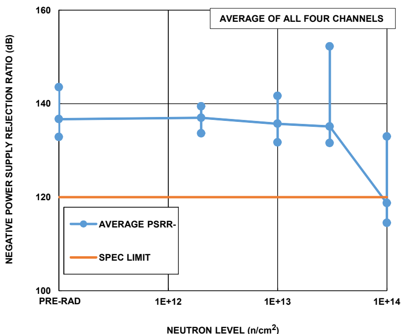
Figure 23. ISL70419SEH negative power supply rejection ratio, average of all four channels, as a function of 1MeV equivalent neutron irradiation at 2 \times 10^{12} \text{n/cm}^2 , 1 \times 10^{13} \text{n/cm}^2 , 3 \times 10^{13} \text{n/cm}^2 , and 1 \times 10^{14} \text{n/cm}^2 . The plot shows the population median, minimum, and maximum at each downpoint. Sample size for each cell was five. The post-total dose irradiation SMD limit is 120dB minimum.
