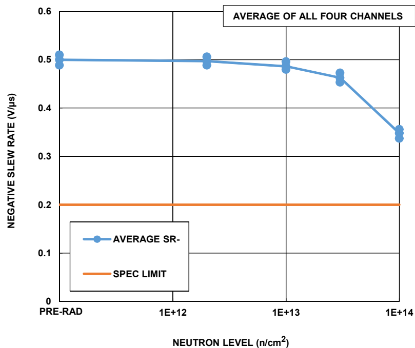
Figure 27. ISL70419SEH negative slew rate, average of all four channels, as a function of 1MeV equivalent neutron irradiation at 2 \times 10^{12} \text{ n/cm}^2 , 1 \times 10^{13} \text{ n/cm}^2 , 3 \times 10^{13} \text{ n/cm}^2 , and 1 \times 10^{14} \text{ n/cm}^2 . The plot shows the population median, minimum, and maximum at each downpoint. Sample size for each cell was five. The post-total dose irradiation SMD limit is 0.2V/μs minimum.
