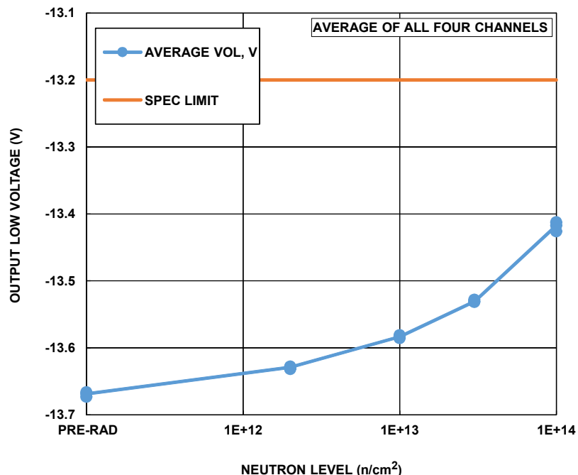
Figure 19. ISL70419SEH output LOW voltage, average of all four channels, as a function of 1MeV equivalent neutron irradiation at 2 \times 10^{12} \text{n/cm}^2 , 1 \times 10^{13} \text{n/cm}^2 , 3 \times 10^{13} \text{n/cm}^2 , and 1 \times 10^{14} \text{n/cm}^2 . The plot shows the population median, minimum, and maximum at each downpoint. Sample size for each cell was five. The post-total dose irradiation SMD limit is -13.2V maximum.
