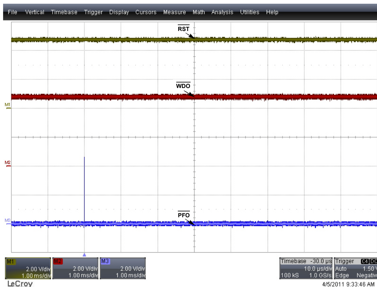
FIGURE 5. TRANSIENT ON \overline{\text{PFO}} ( V_{\text{DD}} = \overline{\text{MR}} = 4.75\text{V} , \text{PFI} = 1.2\text{V} , \overline{\text{WDO}} IS FLOATING)
