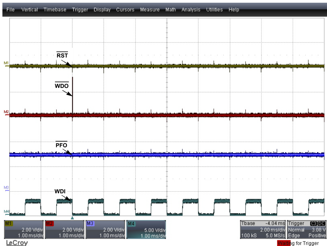
FIGURE 8. TRANSIENT ON \overline{WDO} ( V_{DD} = \overline{MR} = \overline{PFI} = 2.9V , \overline{WDI} IS TOGGLING 0 TO V_{DD} AT 1kHz)
