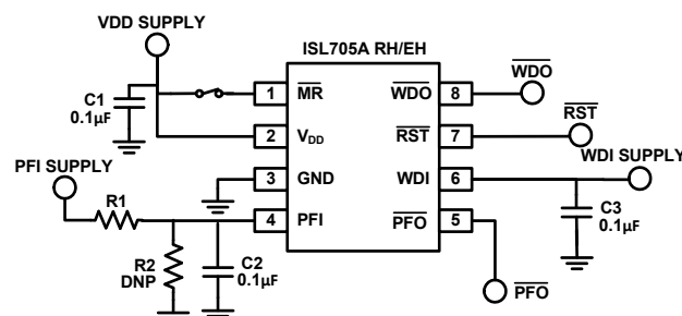
FIGURE 1. ISL705A, ISL706A SEE TEST SCHEMATIC
