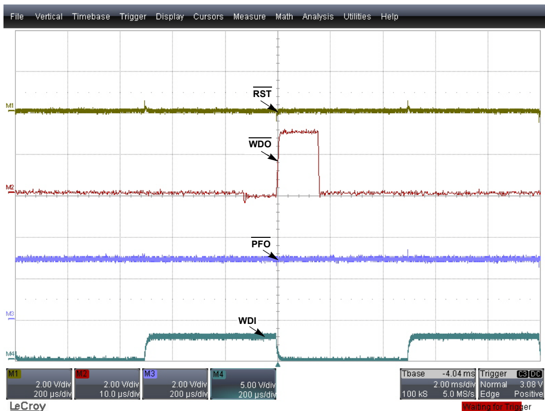
FIGURE 9. SAME \overline{WDO} TRANSIENT AS Figure 8 WITH 10μs PER DIVISION TIME SCALE
