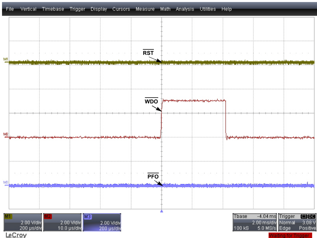
FIGURE 7. SAME \overline{\text{WDO}} TRANSIENT AS Figure 6 WITH 10\mu\text{s} PER DIVISION TIME SCALE
