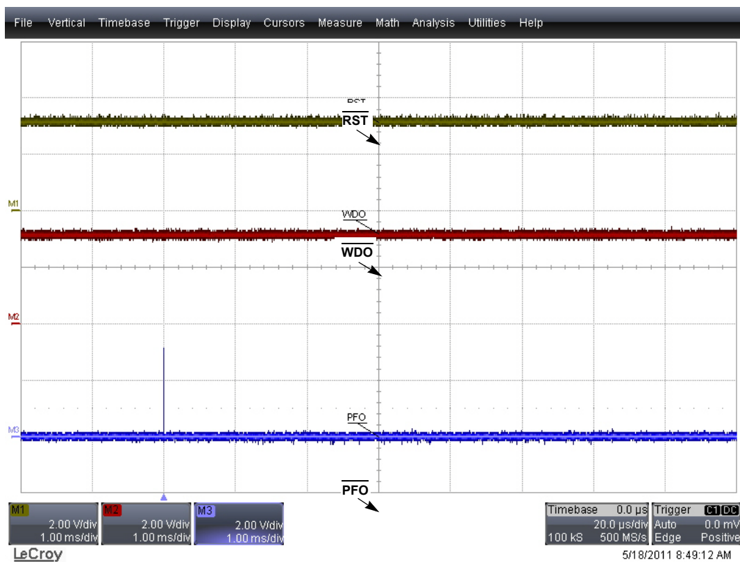
FIGURE 10. TRANSIENT ON \overline{\text{PFO}} ( V_{DD} = \overline{\text{MR}} = 3.15\text{V} , \text{PFI} = 0.576\text{V} , \overline{\text{WDO}} IS FLOATING)
