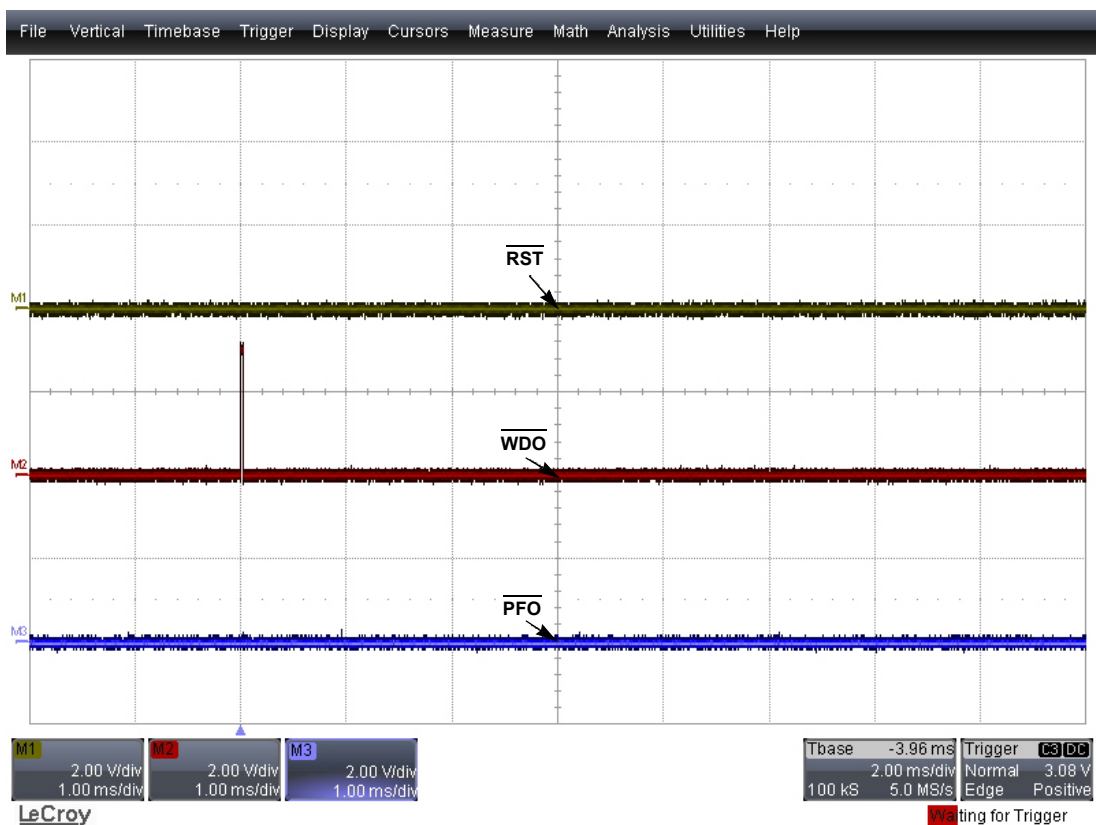
FIGURE 6. TRANSIENTS ON \overline{\text{WDO}} , V_{DD} = \overline{\text{MR}} = 3.0\text{V} , \text{PFI} = 0.57\text{V} , \text{WDI} IS FLOATING
