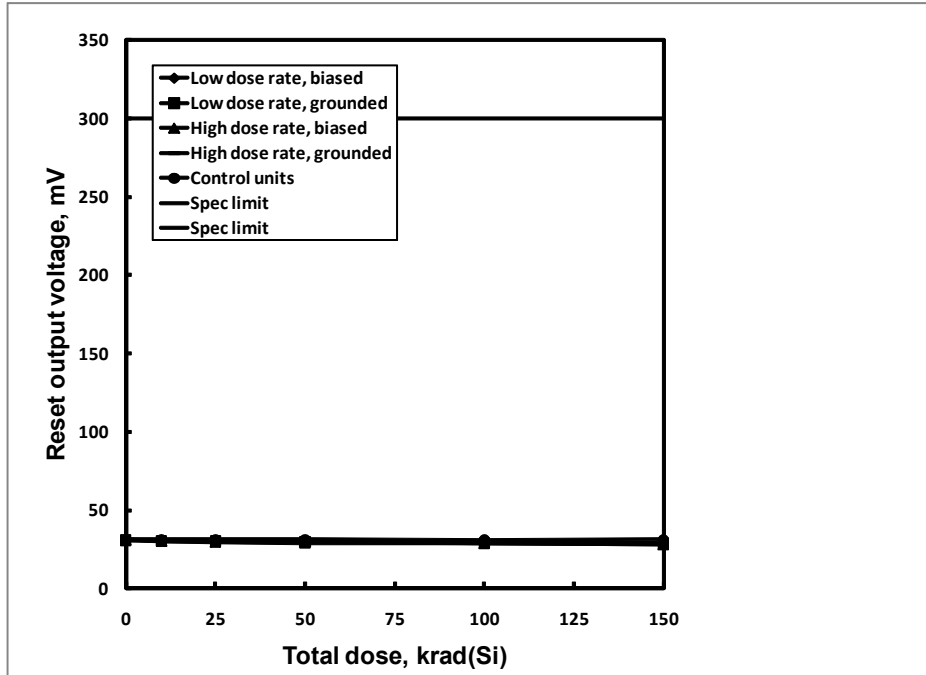
Figure 15. ISL705ARH reset output voltage as a function of total dose irradiation at LDR and HDR for the unbiased (all pins grounded) and the biased (per Figure 2 ) cases. The LDR was 0.01rad(Si)/s and the HDR 85rad(Si)/s. Sample size for each cell was 8, and 4 control units were used. The post-irradiation SMD limit is 300.0mV maximum.
