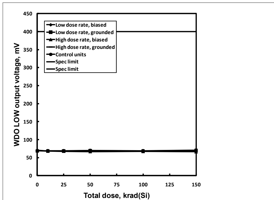
Figure 16. ISL705ARH watchdog output (WDO) low voltage as a function of total dose irradiation at LDR and HDR for the unbiased (all pins grounded) and the biased (per Figure 2 ) cases. The LDR was 0.01rad(Si)/s and the HDR 85rad(Si)/s. Sample size for each cell was 8, and 4 control units were used. The post-irradiation SMD limit is 400.0mV maximum.
