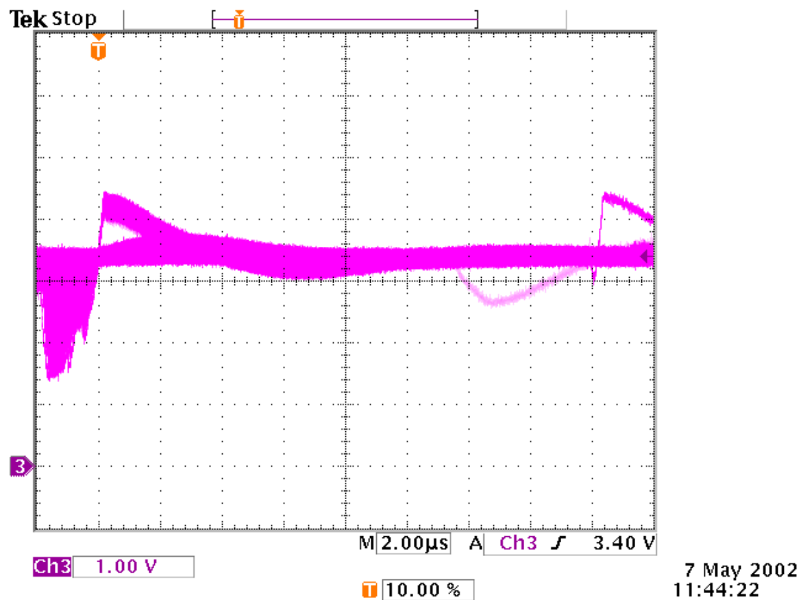
Figure 20: ISL7124SRH SEE response using Kr, LET= 40MeV/mg.cm 2 .
