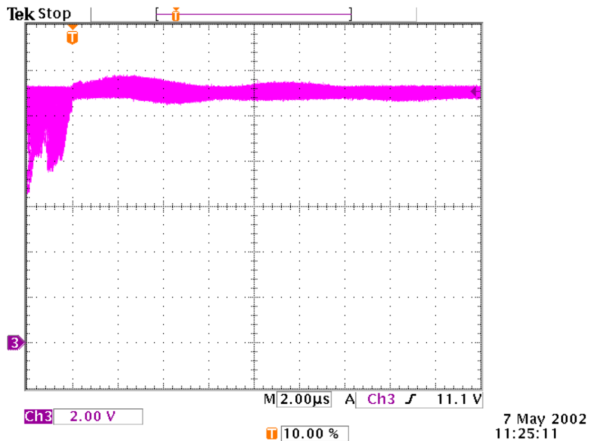
Figure 15: ISL7124SRH SEE response using Kr, LET= 28MeV/mg.cm 2 .
