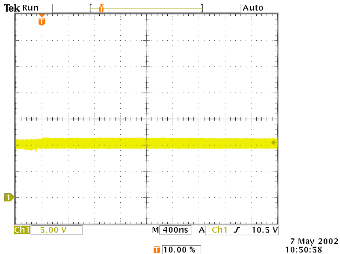
Figure 9: ISL7124SRH SEE response using Kr, LET= 36MeV/mg.cm 2 .
