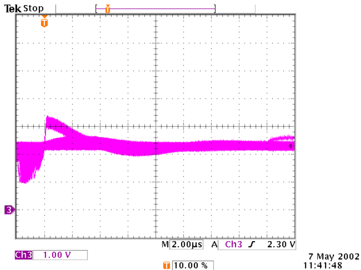
Figure 19: ISL7124SRH SEE response using Kr, LET= 40MeV/mg.cm 2 .
