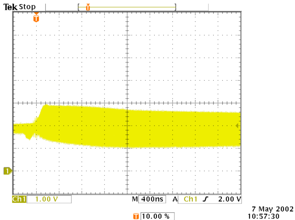
Figure 10: ISL7124SRH SEE response using Kr, LET= 36MeV/mg.cm 2 .
