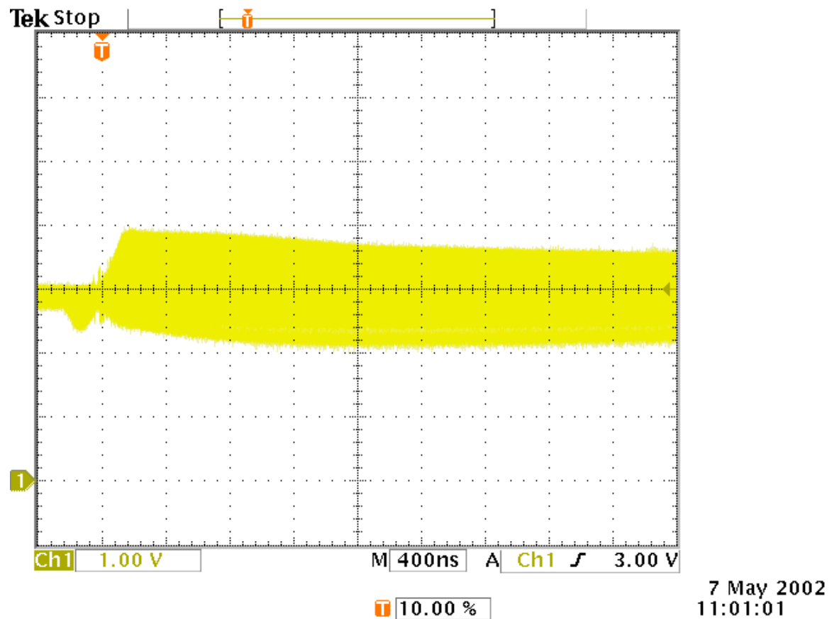
Figure 11: ISL7124SRH SEE response using Kr, LET= 36MeV/mg.cm 2 .
