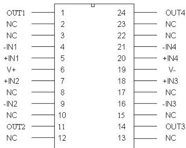
Figure 1: ISL7124SRH SEE Package Pin Diagram
