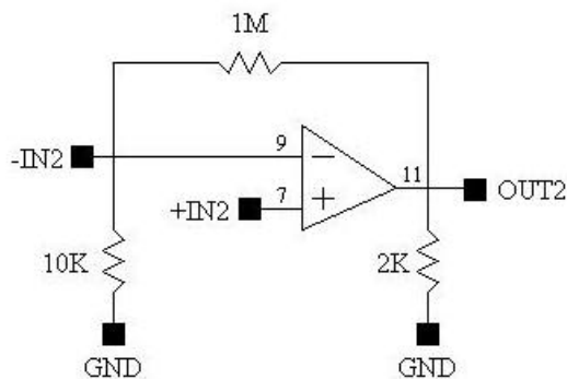
Figure 2: Opamp 2 configured as a non-inverting amplifier with gain = 101.
