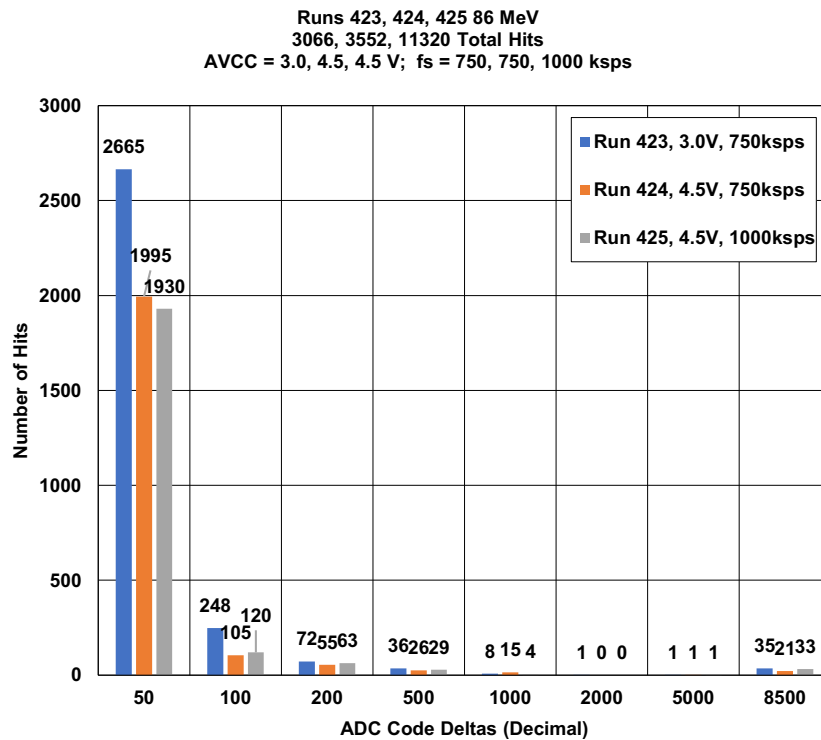
Figure 16. Output Code Delta Histogram for SET for Runs 423, 424, and 425 at 86MeV·cm 2 /mg
