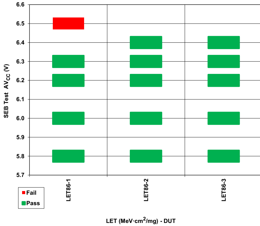
Figure 2. DSEE Testing Pass/Fail Summary - September 2019
