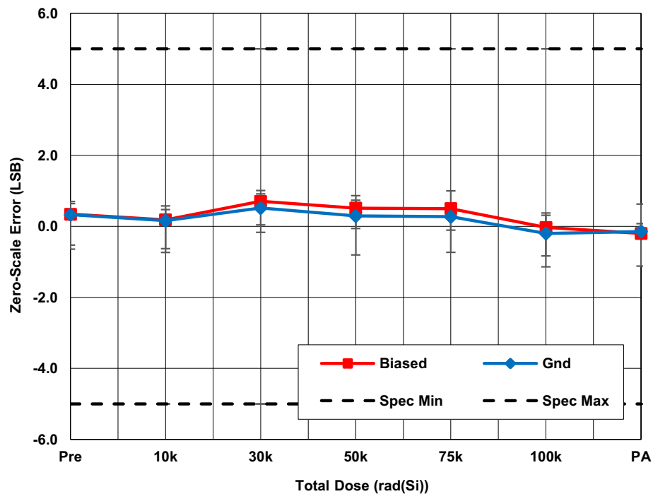
Figure 6. ISL73141SEHMF7 average zero-scale error (Voff) with AV_{CC} = 5V , DV_{CC} = 2.5V , REF = 4.096V , f_{SAMP} = 1Msps , and A_{IN} = GND as a function of LDR irradiation and anneal. The error bars represent the minimum and maximum measured values. The datasheet limits are -5 LSB minimum and 5 LSB maximum.
