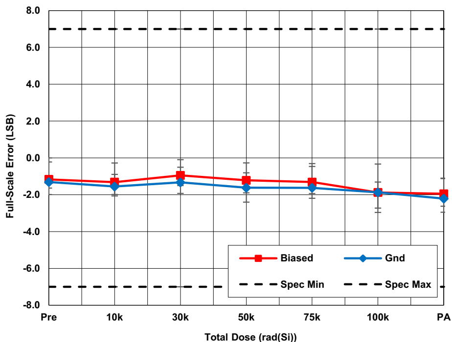
Figure 7. ISL73141SEHMF7 average full-scale error (FSE) with AV_{CC} = 5.0V , DV_{CC} = 2.5V , REF = 4.096V , f_{SAMP} = 1Msps , and A_{IN} = VREF as a function of LDR irradiation and anneal. The error bars represent the minimum and maximum measured values. The datasheet limits are -7 LSB minimum and 7 LSB maximum.
