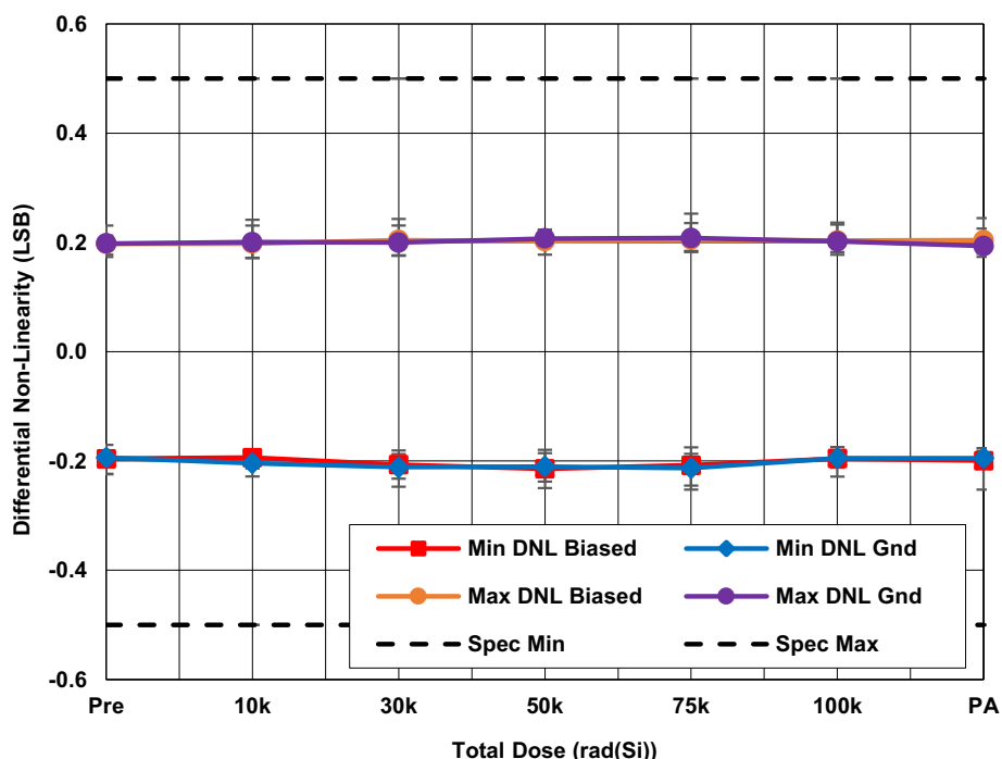
Figure 5. ISL73141SEHMF7 average minimum and maximum differential non-linearity (DNL) with AV_{CC} = 5V , DV_{CC} = 2.5V , REF = 4.096V , f_{SAMP} = 1Msps , and A_{IN} = full-scale sine wave as a function of LDR irradiation and anneal. The error bars represent the minimum and maximum measured values. The datasheet limits are -0.5 LSB minimum and 0.5 LSB maximum.
