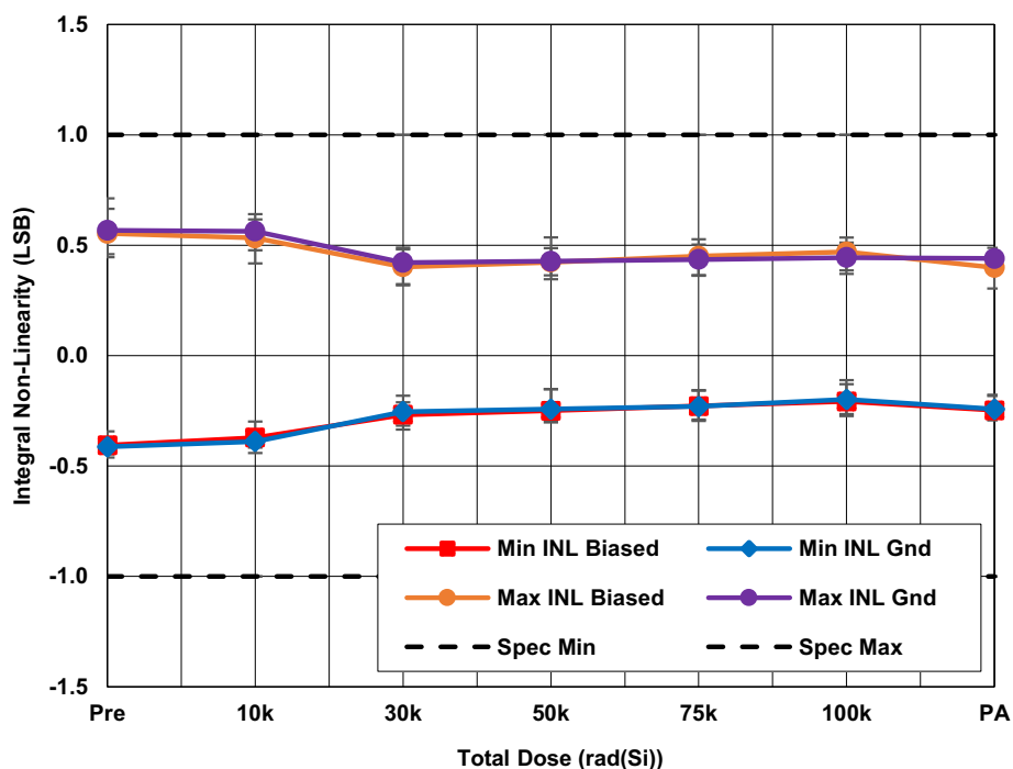
Figure 4. ISL73141SEHMF7 average minimum and maximum integral non-linearity (INL) with AV_{CC} = 5V , DV_{CC} = 2.5V , REF = 4.096V , f_{SAMP} = 1Msps , and A_{IN} = full-scale sine wave as a function of LDR irradiation and anneal. The error bars represent the minimum and maximum measured values. The datasheet limits are -1 LSB minimum and 1 LSB maximum.
