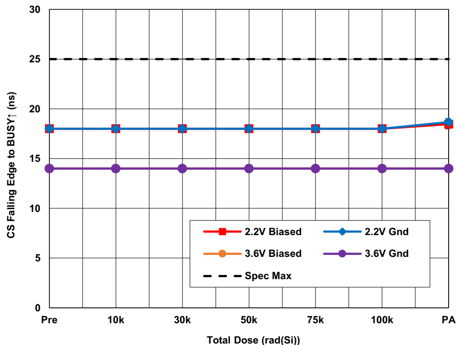
Figure 28. ISL73141SEHMF7 average \overline{\text{CS}} falling edge to BUSY rising edge ( t_{\text{BUSYLH}} ) with \text{AV}_{\text{CC}} = 4.5\text{V} , \text{DV}_{\text{CC}} = 2.2\text{V} and \text{AV}_{\text{CC}} = 5.5\text{V} , \text{DV}_{\text{CC}} = 3.6\text{V} , \text{REF} = 4.096\text{V} , f_{\text{SAMP}} = 1\text{Msps} , \text{A}_{\text{IN}} = -1\text{dbFS} and \text{C}_{\text{L}} = 10\text{pF} as a function of LDR irradiation and anneal. The error bars represent the minimum and maximum measured values. The datasheet limit is 25ns maximum.
