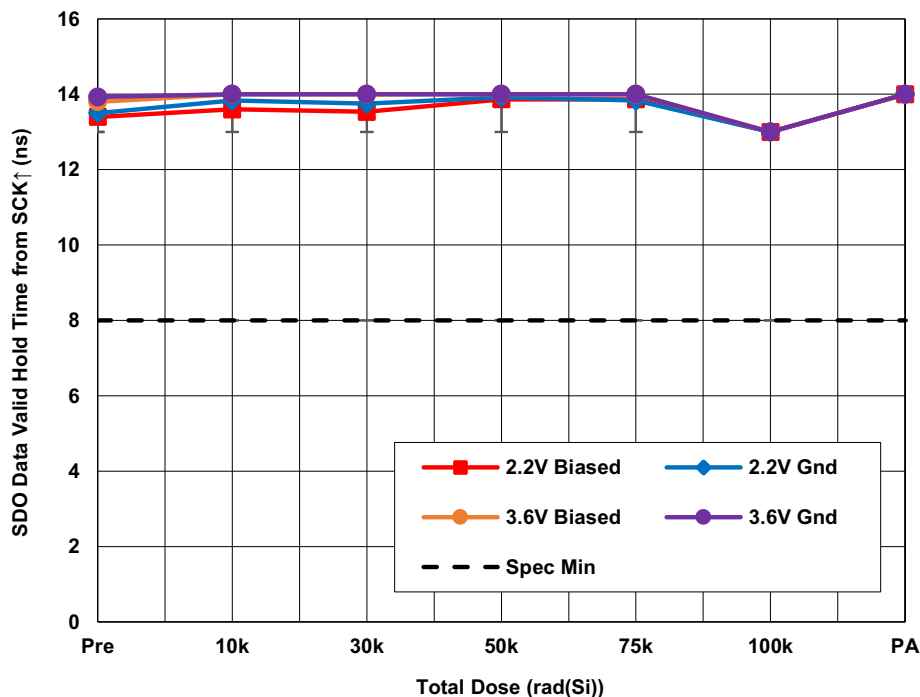
Figure 30. ISL73141SEHMF7 average SDO data valid hold time from SCK rising edge ( t_{HSDOV} ) with AV_{CC} = 4.5V , DV_{CC} = 2.2V and AV_{CC} = 5.5V , DV_{CC} = 3.6V , REF = 4.096V , f_{SAMP} = 1Msps , A_{IN} = -1dbFS , and C_L = 10pF as a function of LDR irradiation and anneal. The error bars represent the minimum and maximum measured values. The datasheet limit is 8ns minimum.
