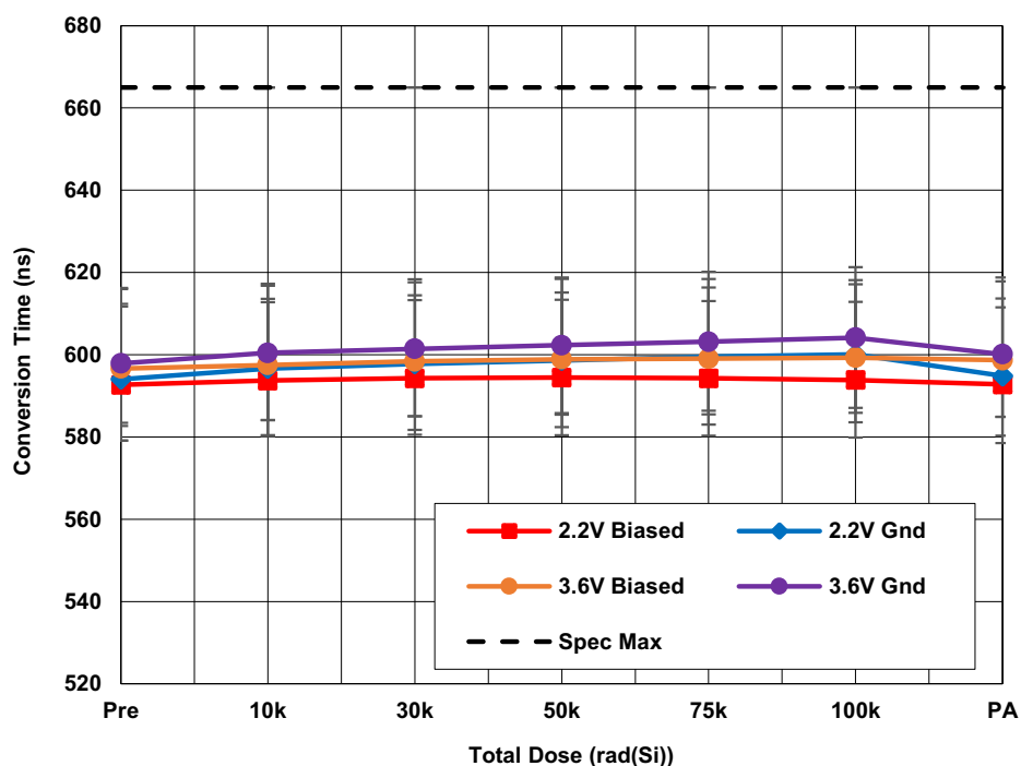
Figure 27. ISL73141SEHMF7 average conversion time ( t_{CONV} ) with AV_{CC} = 4.5V , DV_{CC} = 2.2V and AV_{CC} = 5.5V , DV_{CC} = 3.6V , REF = 4.096V , f_{SAMP} = 1Msps , and A_{IN} = -1dbFS as a function of LDR irradiation and anneal. The error bars represent the minimum and maximum measured values. The datasheet limit is 665ns maximum.
