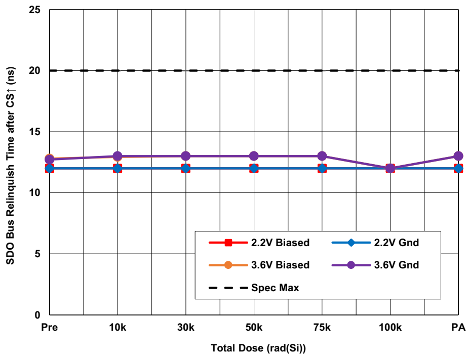
Figure 32. ISL73141SEHMF7 average SDO bus relinquish time after \overline{CS} rising edge ( t_{DCSHSDOZ} ) with AV_{CC} = 4.5V , DV_{CC} = 2.2V and AV_{CC} = 5.5V , DV_{CC} = 3.6V , REF = 4.096V , f_{SAMP} = 1Msps , A_{IN} = -1dbFS , and C_L = 10pF as a function of LDR irradiation and anneal. The error bars represent the minimum and maximum measured values. The datasheet limit is 20ns maximum.
