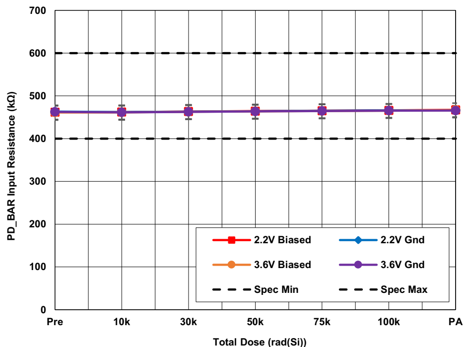
Figure 26. ISL73141SEHMF7 average \overline{PD} input resistance ( R_{INPDL} ) with AV_{CC} = 5V , DV_{CC} = 2.2V and 3.6V and REF = 4.096V as a function of LDR irradiation and anneal. The error bars represent the minimum and maximum measured values. The datasheet limits are 400 k\Omega minimum and 600 k\Omega maximum.
