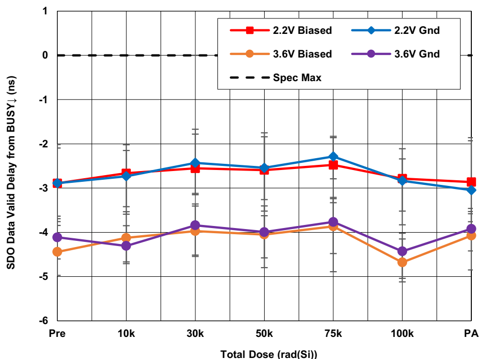
Figure 29. ISL73141SEHMF7 average SDO data valid delay from BUSY falling edge ( t_{\text{DBUSYLSDOV}} ) with \text{AV}_{\text{CC}} = 4.5\text{V} , \text{DV}_{\text{CC}} = 2.2\text{V} and \text{AV}_{\text{CC}} = 5.5\text{V} , \text{DV}_{\text{CC}} = 3.6\text{V} , \text{REF} = 4.096\text{V} , f_{\text{SAMP}} = 1\text{Msps} , \text{A}_{\text{IN}} = -1\text{dbFS} and \text{C}_{\text{L}} = 10\text{pF} as a function of LDR irradiation and anneal. The error bars represent the minimum and maximum measured values. The datasheet limit is 0ns maximum.
