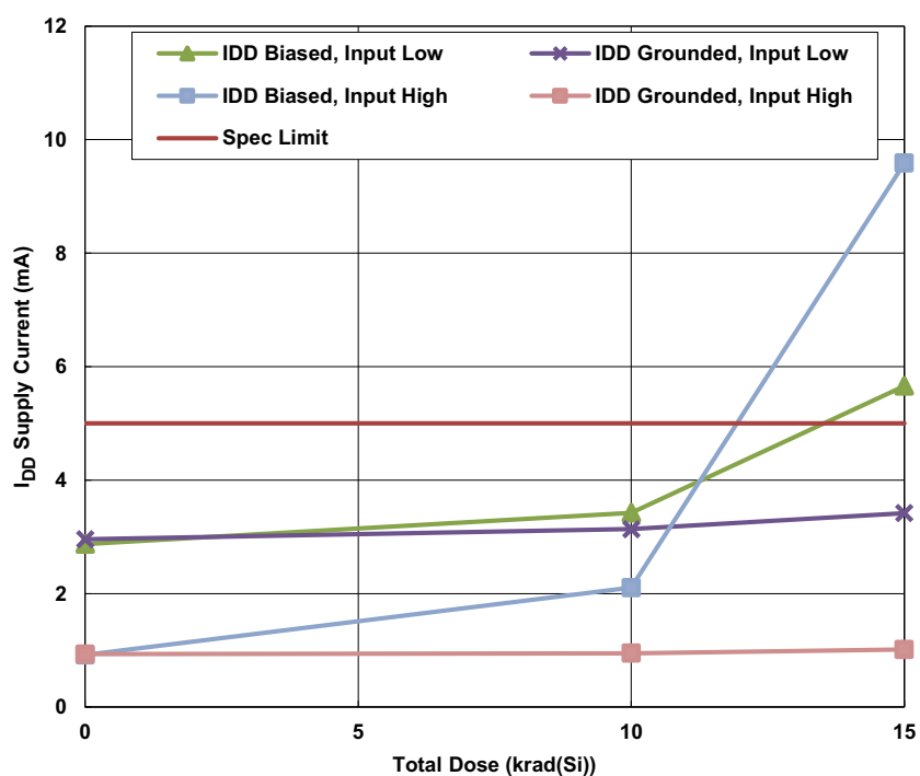
Figure 3. ISL7457SRH quad CMOS driver positive power supply current at 5V supply, input low and high cases, as a function of LDR total dose irradiation for the unbiased (grounded) and biased cases. The dose rate was 0.01rad(Si)/s. Sample sizes were two each for the unbiased and biased groups. The post-radiation SMD limit is 5mA maximum.
