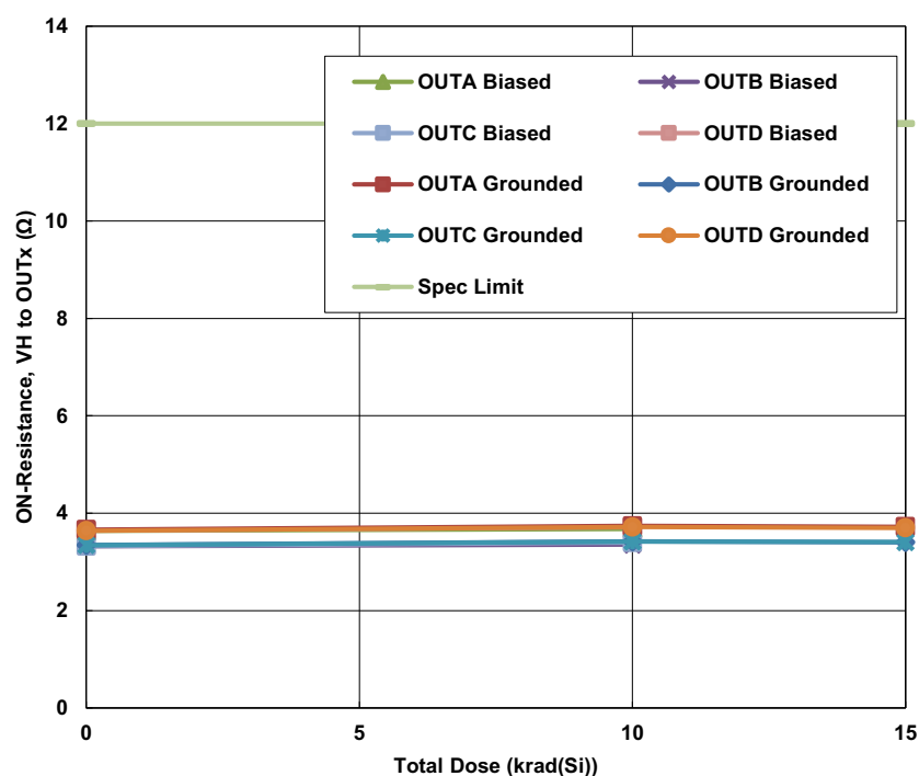
Figure 9. ISL7457SRH quad CMOS driver ON-resistance, VH to OUTx at 5V supply, as a function of LDR total dose irradiation for the unbiased (grounded) and biased cases. The dose rate was 0.01rad(Si)/s. Sample sizes were two each for the unbiased and biased groups. The post-radiation SMD limit is 12Ω maximum.
