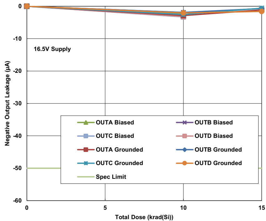
Figure 6. ISL7457SRH quad CMOS driver negative output leakage current at 16.5V supply as a function of LDR total dose irradiation for the unbiased (grounded) and biased cases. The dose rate was 0.01\text{rad}(\text{Si})/\text{s} . Sample sizes were two each for the unbiased and biased groups. The post-radiation SMD limit is -50\mu\text{A} minimum.
