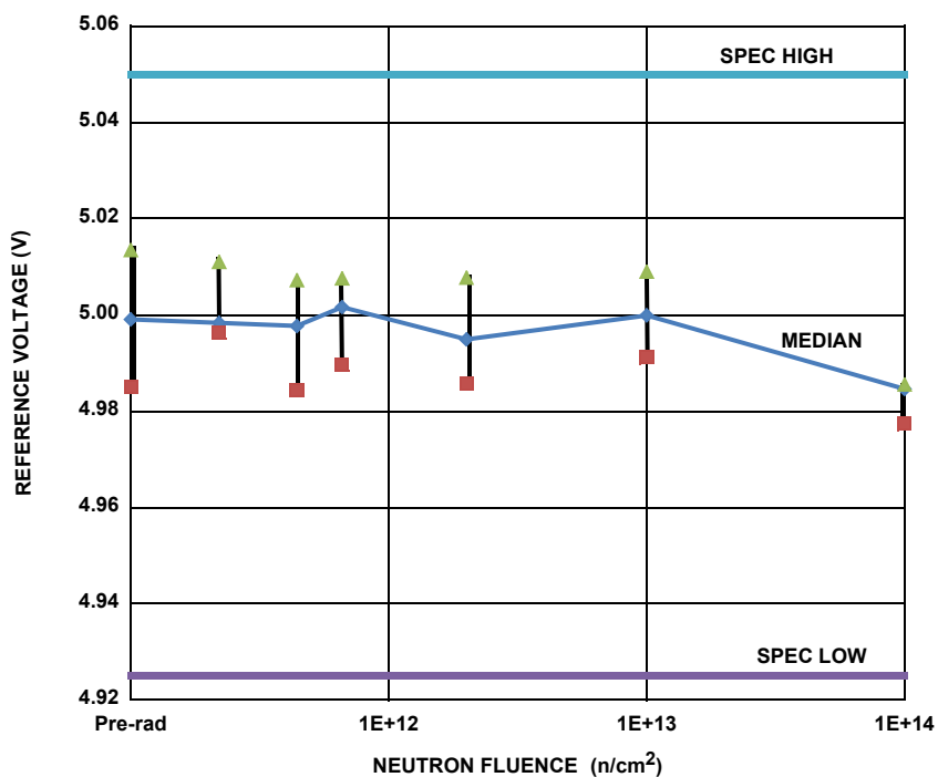
FIGURE 6. ISL78845ASEH reference voltage accuracy as a function of neutron irradiation, showing the median, minimum and maximum of the populations at each level. Neutron fluences and sample sizes (in parentheses) were 2.2 \times 10^{11} \text{ n/cm}^2 (6 samples), 4.4 \times 10^{11} \text{ n/cm}^2 (6 samples), 6.6 \times 10^{11} \text{ n/cm}^2 (6 samples), 1 \times 10^{12} \text{ n/cm}^2 (3 samples), 1 \times 10^{13} \text{ n/cm}^2 (3 samples) and 1 \times 10^{14} \text{ n/cm}^2 (3 samples). The SMD limits are 4.925V to 5.050V.
