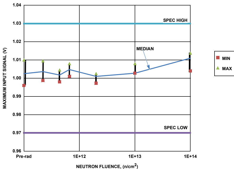
FIGURE 10. ISL78845ASEH current sense maximum input signal as a function of neutron irradiation, showing the median, minimum and maximum of the populations at each level. Neutron fluences and sample sizes (in parentheses) were 2.2 \times 10^{11} \text{ n/cm}^2 (6 samples), 4.4 \times 10^{11} \text{ n/cm}^2 (6 samples), 6.6 \times 10^{11} \text{ n/cm}^2 (6 samples), 1 \times 10^{12} \text{ n/cm}^2 (3 samples), 1 \times 10^{13} \text{ n/cm}^2 (3 samples) and 1 \times 10^{14} \text{ n/cm}^2 (3 samples). The SMD limits are 0.97V to 1.03V.
