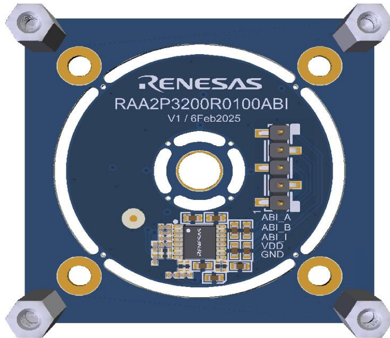
Figure 1. Sensor Board
