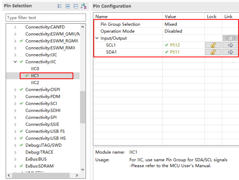
Figure 3-23 IIC1 Pin Configuration for MIPI camera of EK-RA8D2
