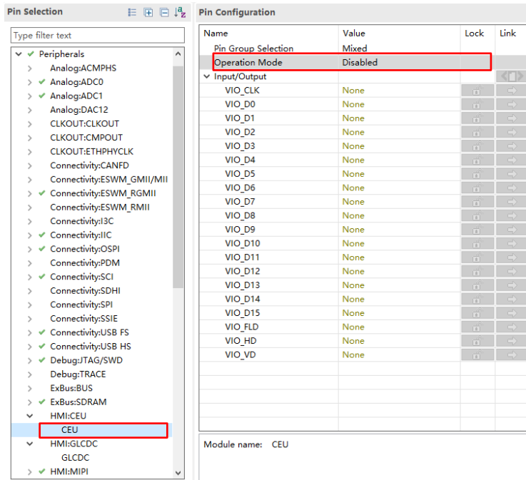
Figure 3-17 CEU Pin Configuration for LCD Module of EK-RA8D2
