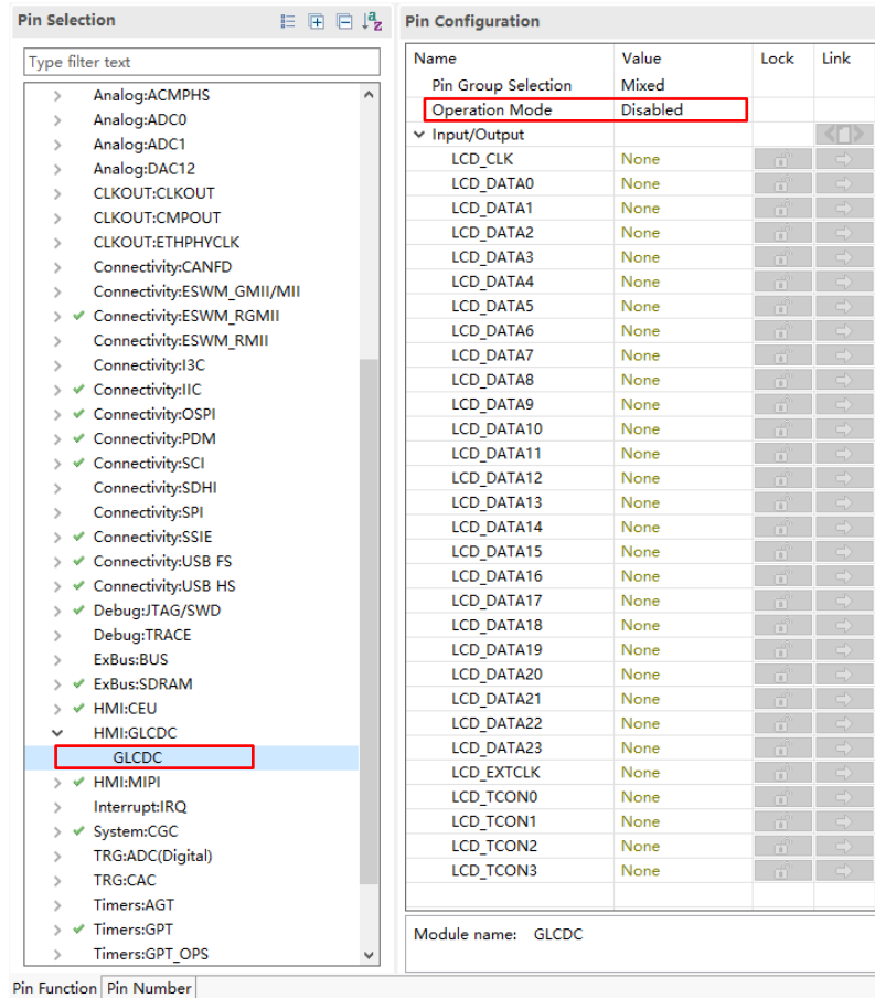
Figure 3-31 GLCDC Pin Configuration for Parallel Camera of EK-RA8P1
