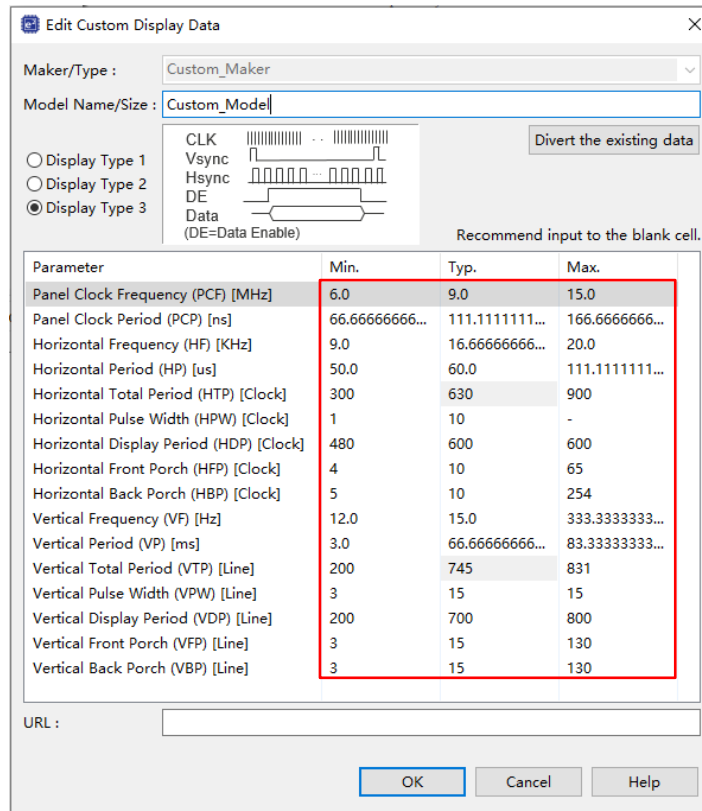
Figure 1-5 Edit the Custom LCD Parameters
