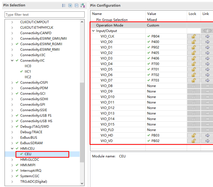
Figure 3-19 CEU Pin Configuration for Parallel Camera of EK-RA8D2
