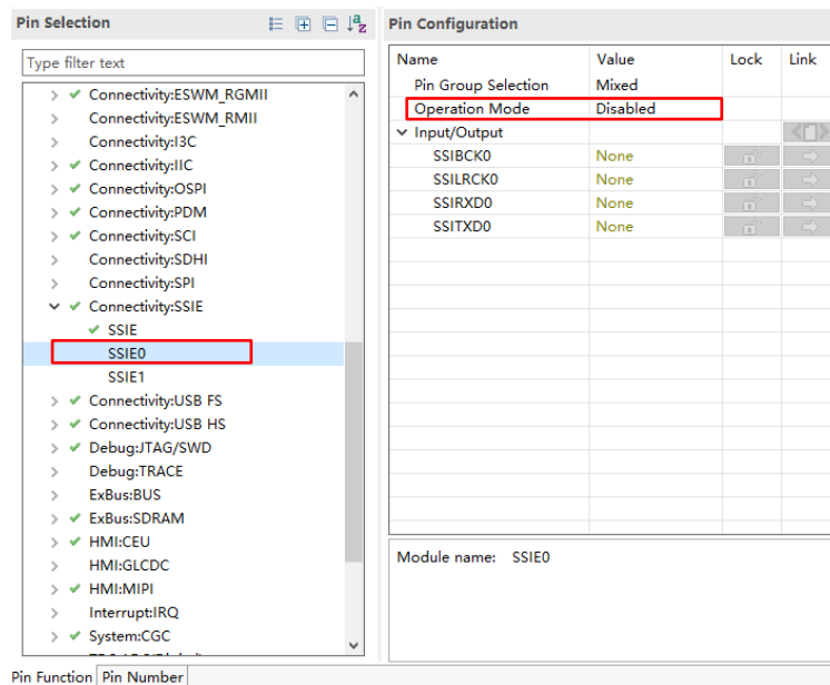
Figure 3-30 SSIE0 Pin Configuration for Parallel Camera of EK-RA8P1
