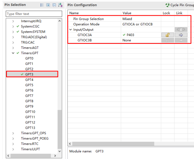
Figure 3-13 GPT3 Pin Configuration for EK-RA8D1
