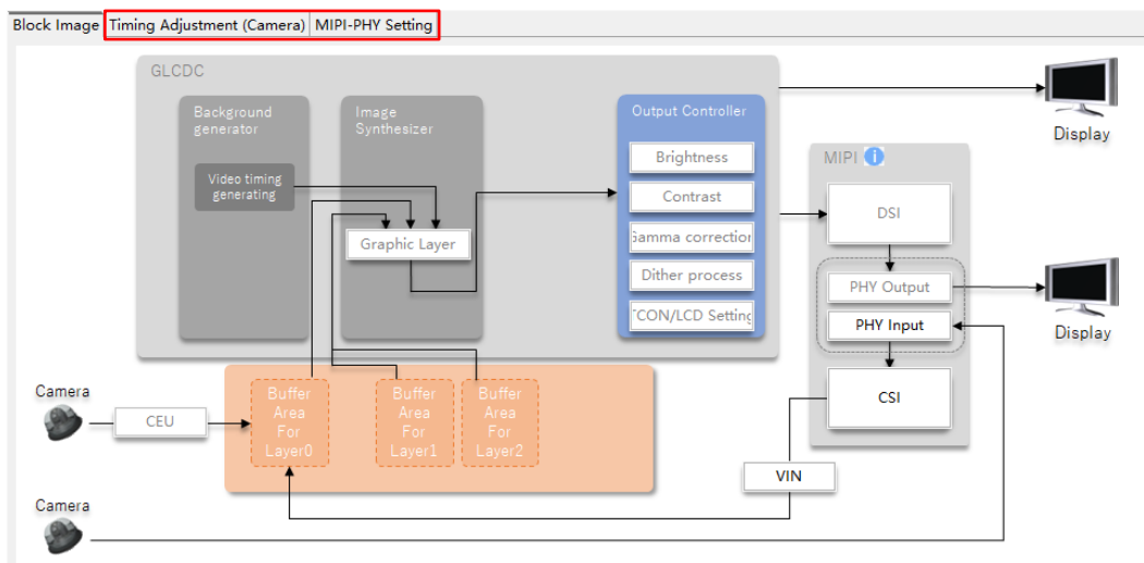
Figure 1-3 RA8P1 and RA8D2 MIPI PHY, MIPI CSI and Video Input Module (VIN) Setting
