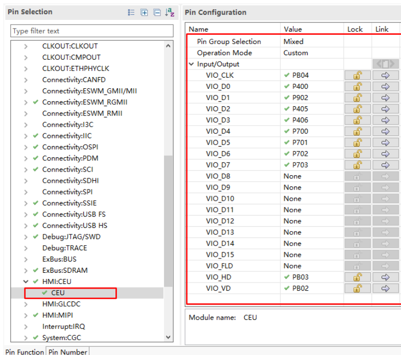
Figure 3-32 CEU Pin Configuration for Parallel Camera of EK-RA8P1
