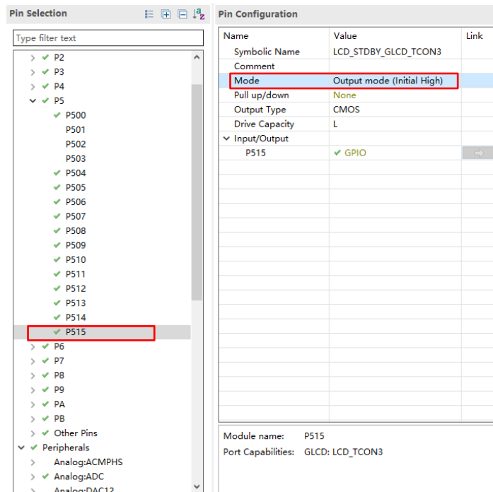
Figure 3-26 "LCD_TCON3" Pin Configuration for EK-RA8E2
