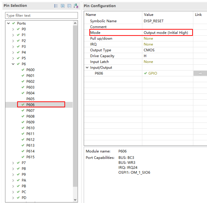
Figure 3-16 "DISP_RESET" Pin Configuration for EK-RA8D2
