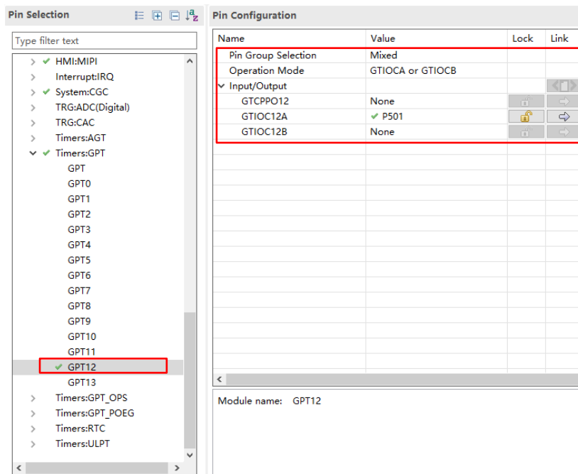
Figure 3-37 GPT12 Pin Configuration for MIPI camera of EK-RA8P1
