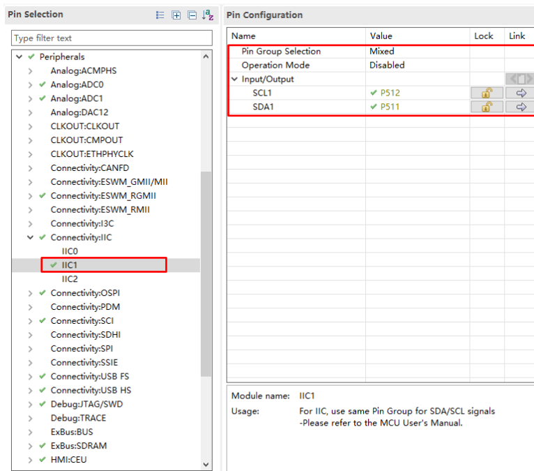
Figure 3-20 IIC1 Pin Configuration for Parallel Camera of EK-RA8D2
