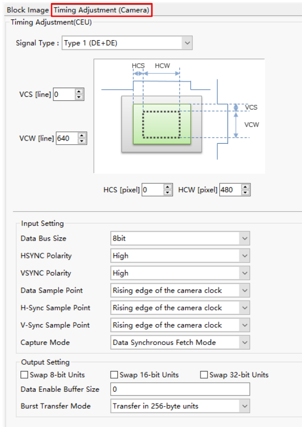
Figure 1-2 RA8D2 Capture Engine Unit (CEU) Setting
