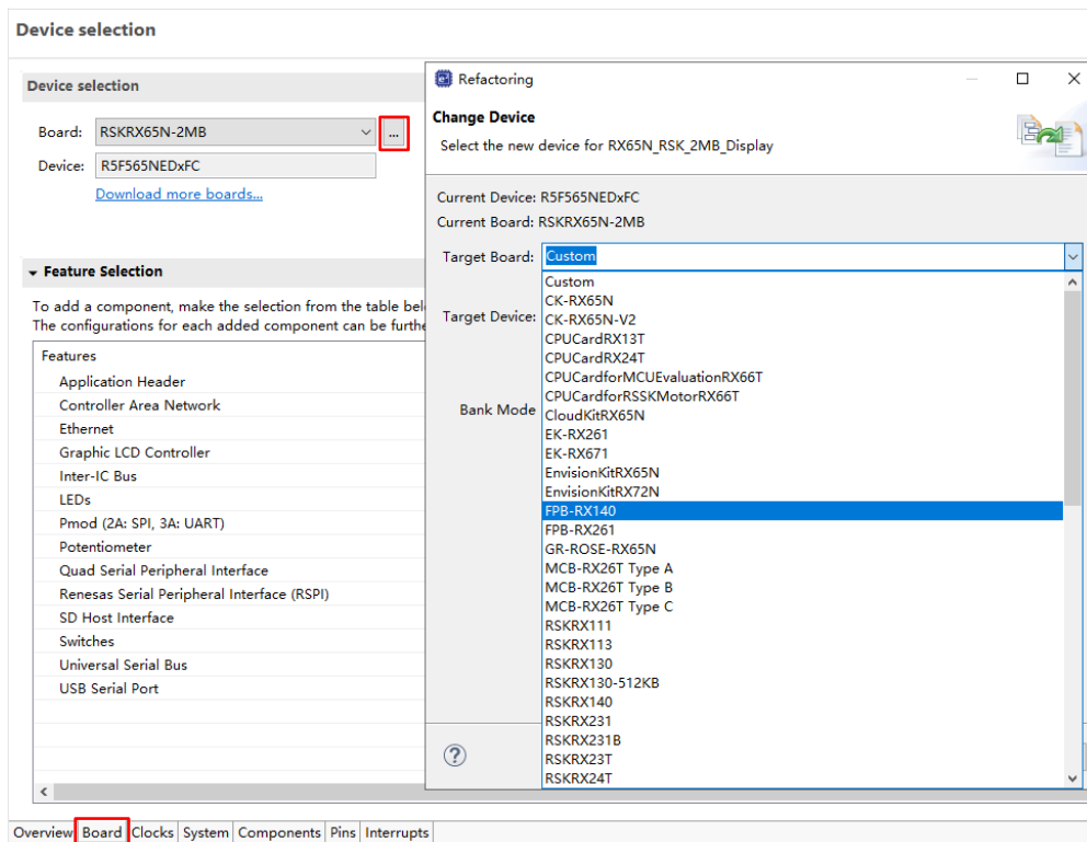
Figure 3-40 [Change Board] Operation in Smart Configurator
