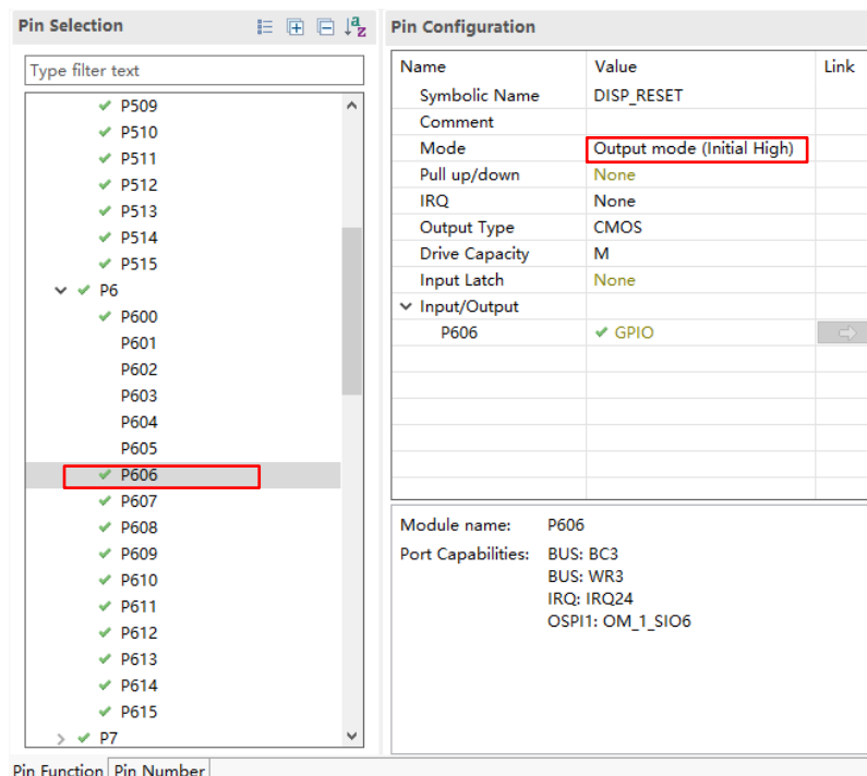
Figure 3-28 "DISP_RESET" Pin Configuration for EK-RA8P1
