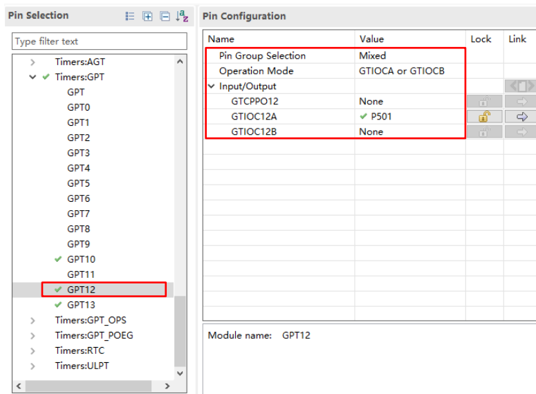
Figure 3-24 GPT12 Pin Configuration for MIPI camera of EK-RA8D2
