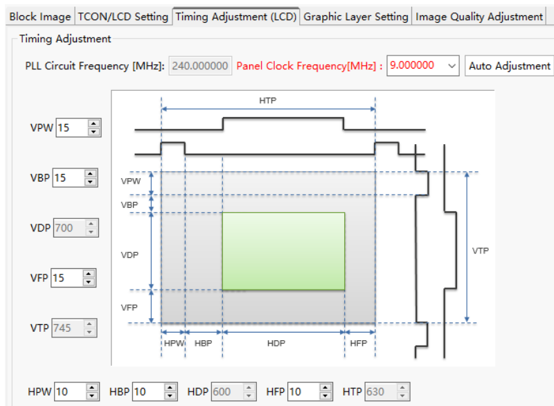
Figure 1-6 Reload Custom LCD Parameters in GUI
