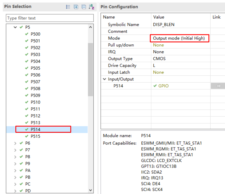
Figure 3-27 "DISP_BLEN" Pin Configuration for EK-RA8P1
