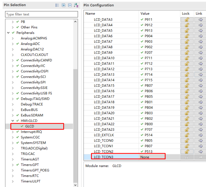
Figure 3-25 GLCD Pin Configuration for EK-RA8E2
