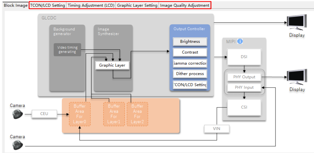
Figure 1-1 RA8D2 Graphics LCD Controller (GLCDC) Setting
