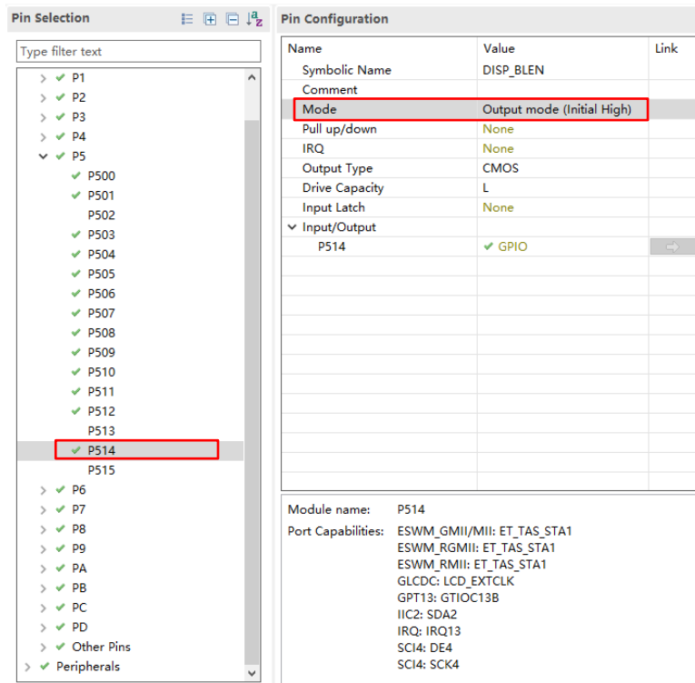
Figure 3-15 "DISP_BLEN" Pin Configuration for EK-RA8D2
