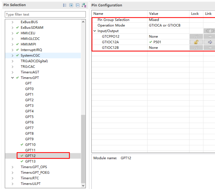
Figure 3-21 GPT12 Pin Configuration for Parallel Camera of EK-RA8D2
