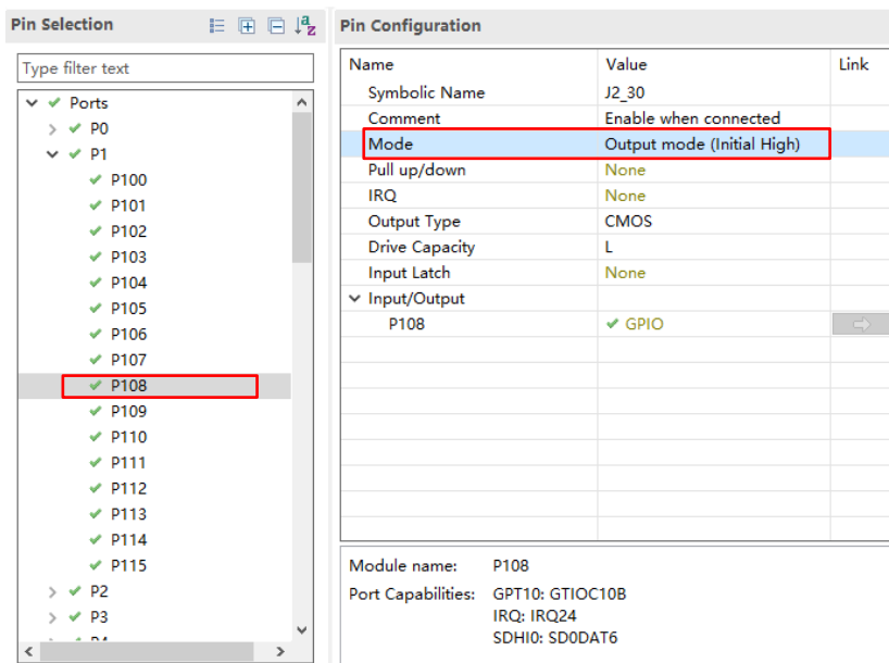
Figure 3-22 P108 Pin Configuration for MIPI camera of EK-RA8D2
