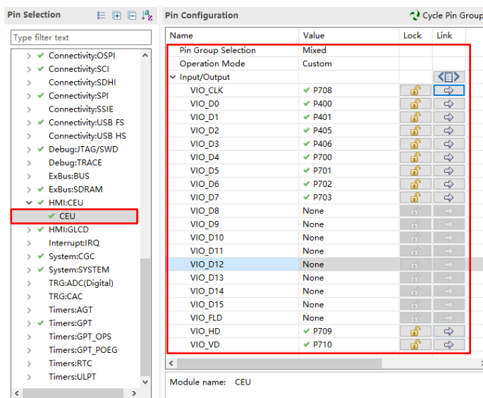
Figure 3-12 CEU Pin Configuration for EK-RA8D1
