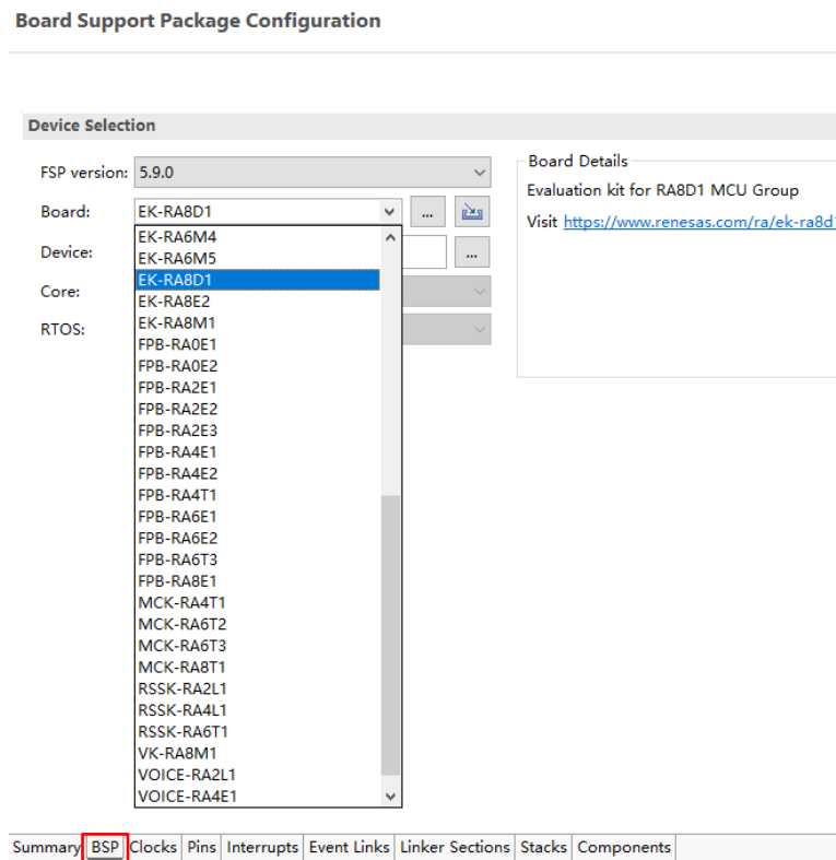
Figure 3-39 [Change Board] Operation in FSP
