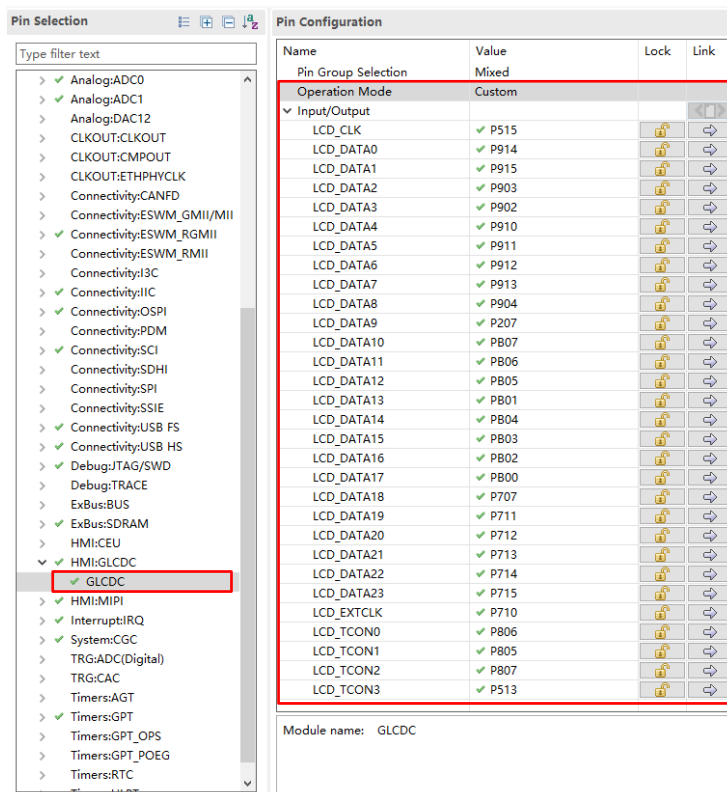
Figure 3-18 GLCDC Pin Configuration for EK-RA8D2
