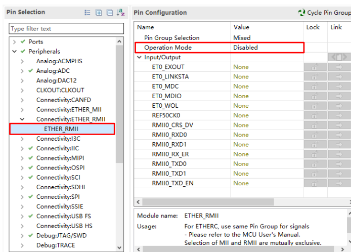
Figure 3-11 ETHER_RMII Pin Configuration for EK-RA8D1
