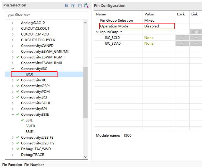
Figure 3-29 I3C0 Pin Configuration for Parallel Camera of EK-RA8P1
