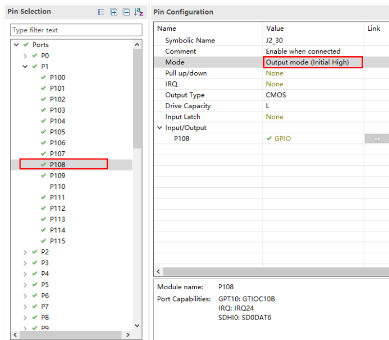
Figure 3-35 P108 Pin Configuration for MIPI camera of EK-RA8P1
