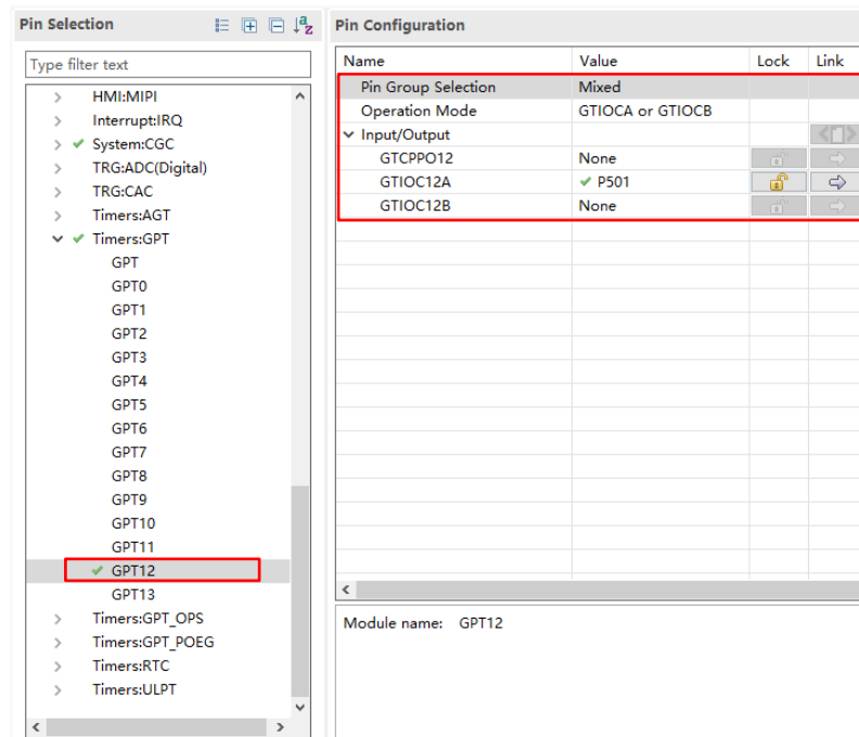
Figure 3-34 GPT12 Pin Configuration for parallel camera of EK-RA8P1
