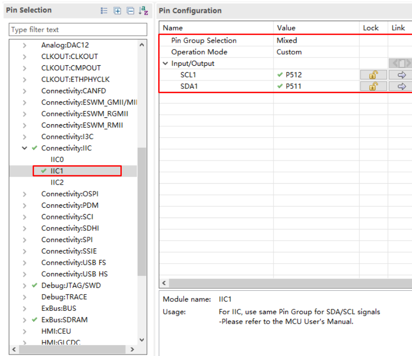
Figure 3-33 IIC1 Pin Configuration for Parallel Camera of EK-RA8P1
