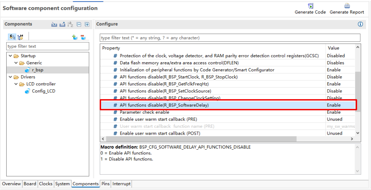
Figure 3-6 Enable R_BSP_SoftwareDelay function
