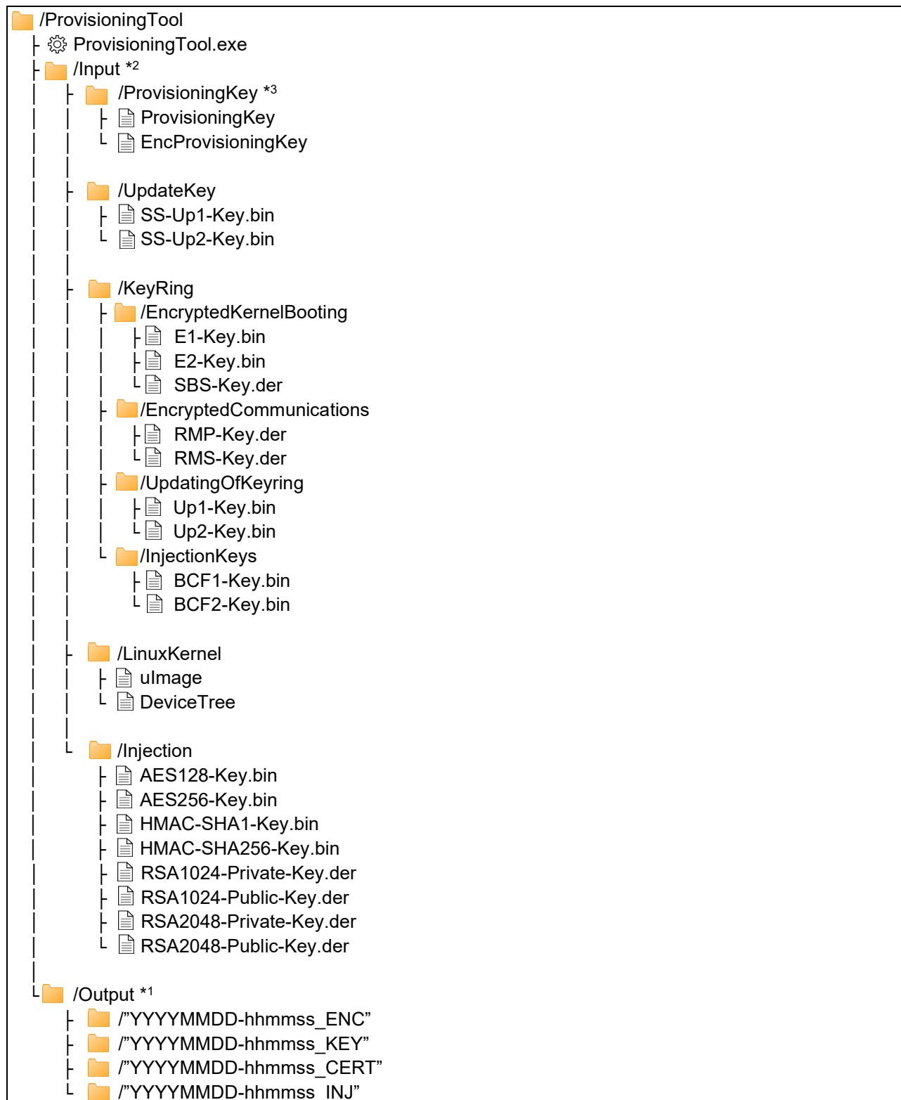
Figure 11-1 Configuration of Files for Provisioning Tool
