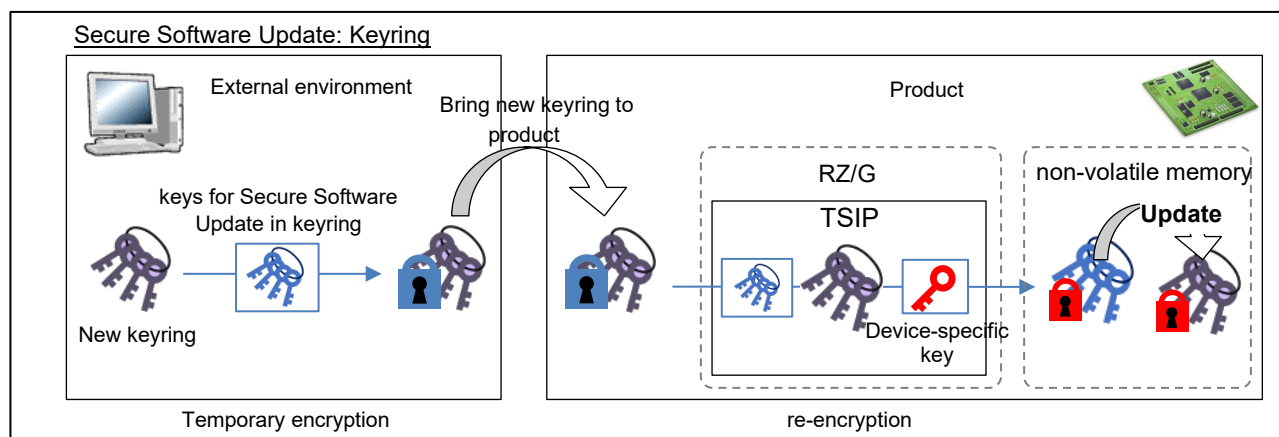
Figure 9-1 Schematic View of Secure Software Update (Keyring)
