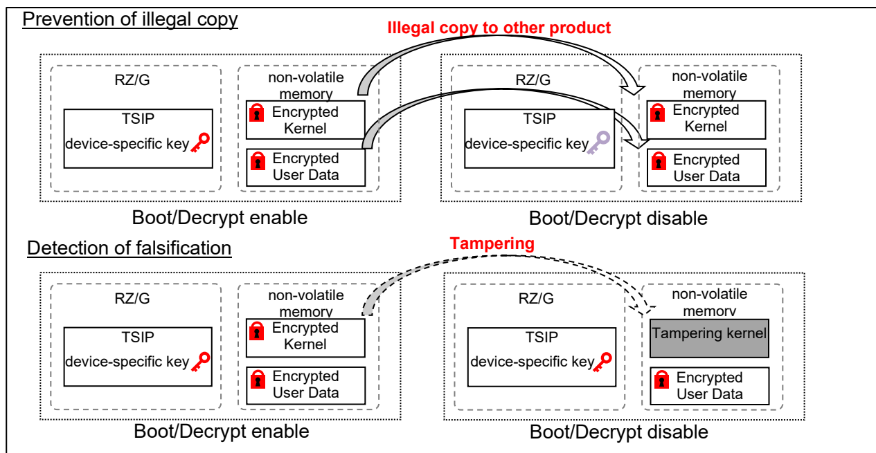
Figure 1-2 Schematic View of Encryption with Device-Specific Key
