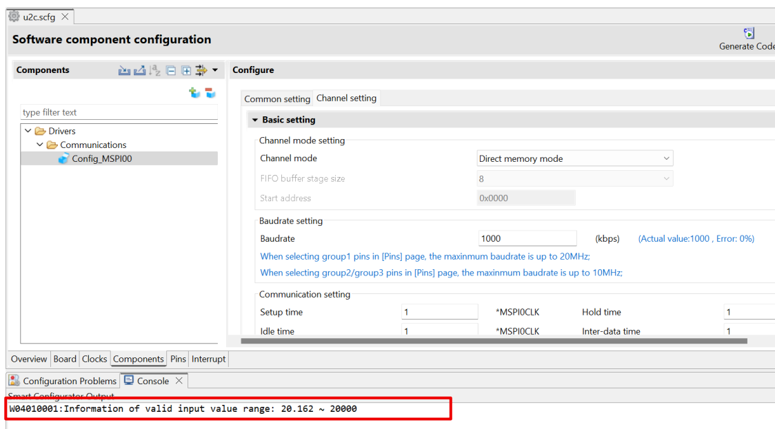
Figure 3-2 RH850/U2C MSPI Master baudrate range
