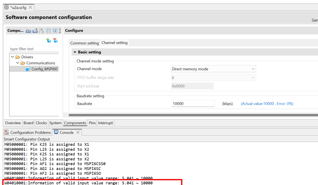
Figure 3-1 RH850/U2A MSPI Master baudrate range
