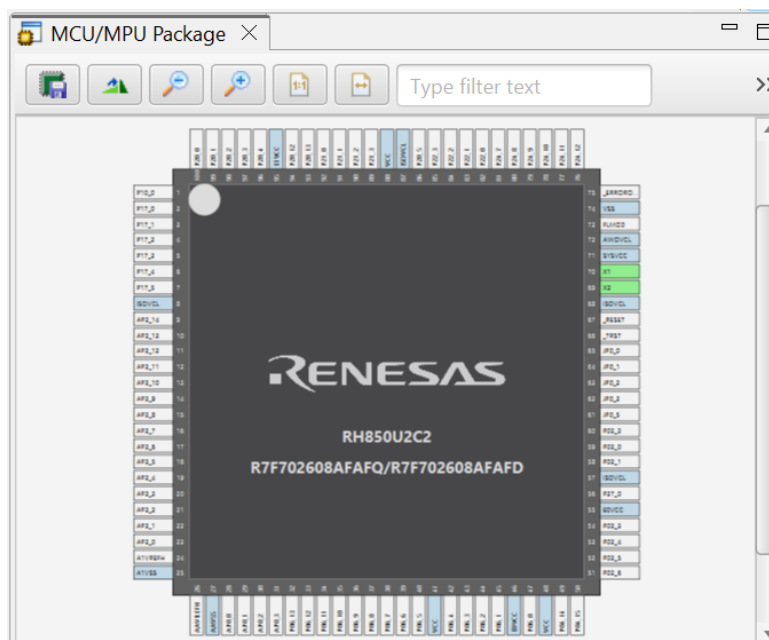
Figure 3-5 Correct MCU package
