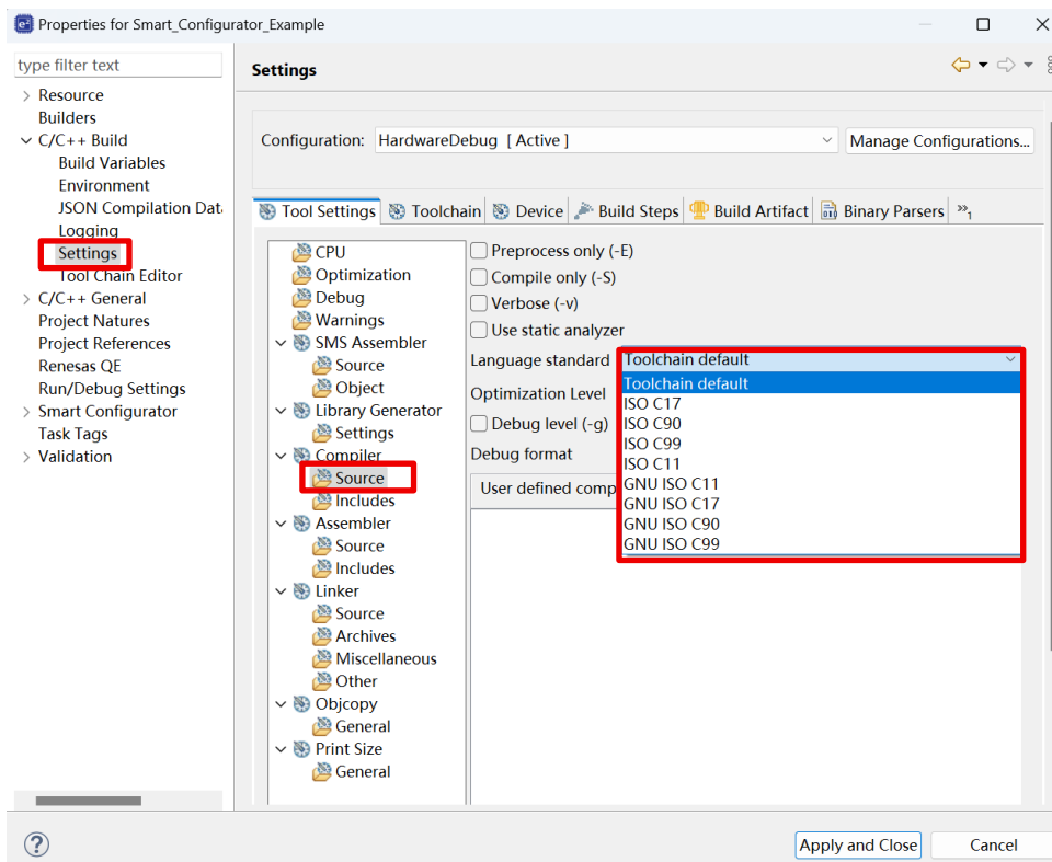
Figure 3-2 The property of “Language standard” in LLVM project
