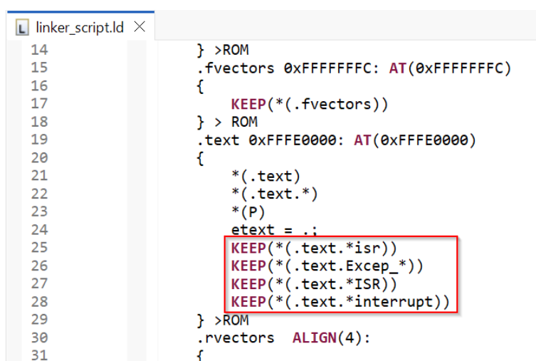
Figure 3-1 KEEP information in linker script file
