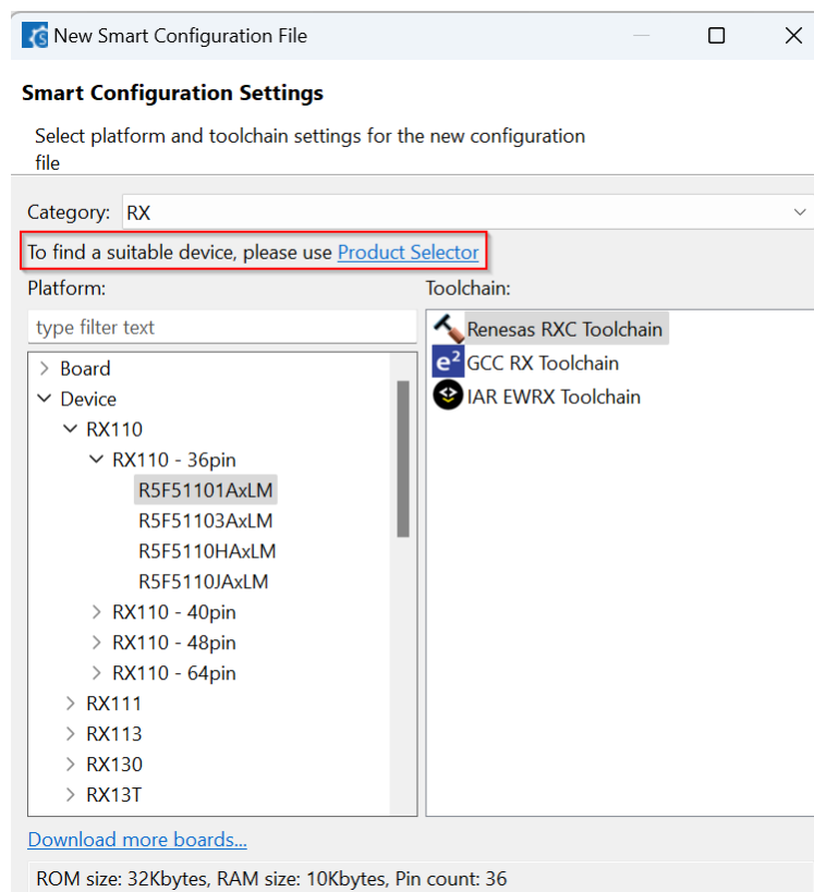
Figure 2-1 The link to Product Selector
