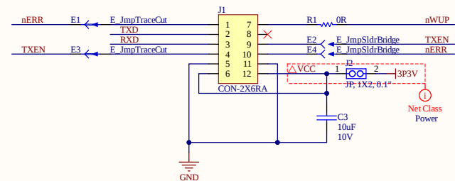
PMOD Interface Type 3A (expanded UART)
