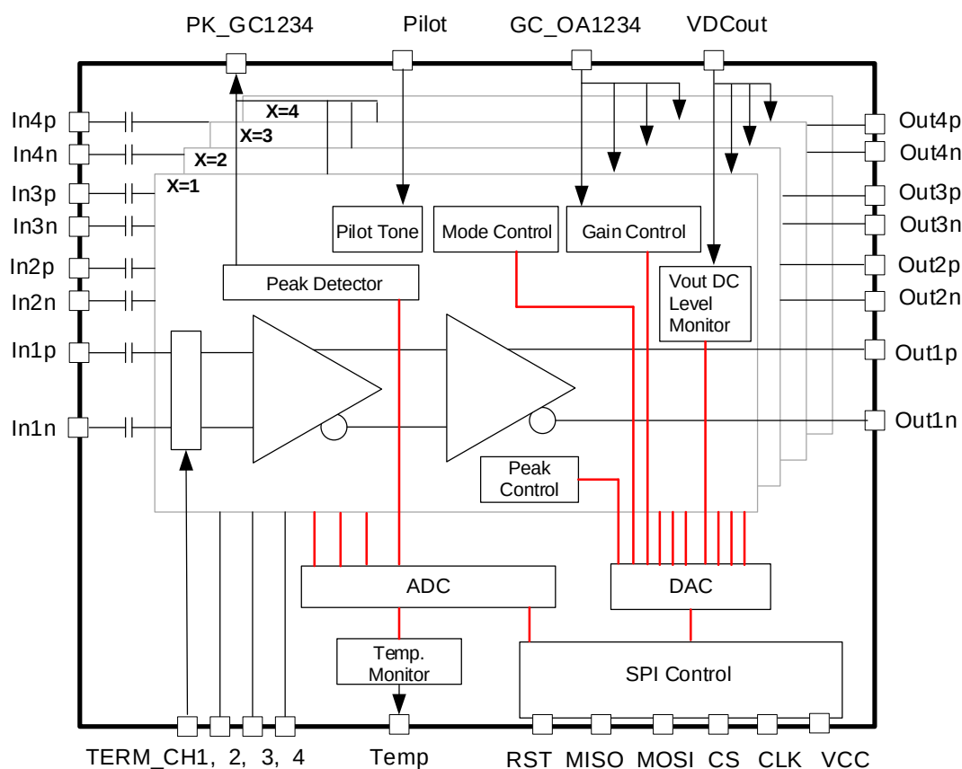
Figure 1. Block Diagram
