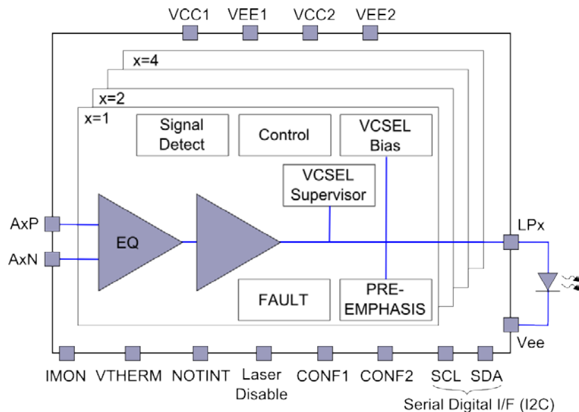
Figure 1. Block Diagram
