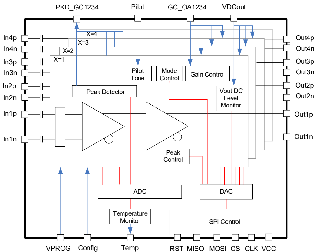
Figure 1. Block Diagram
