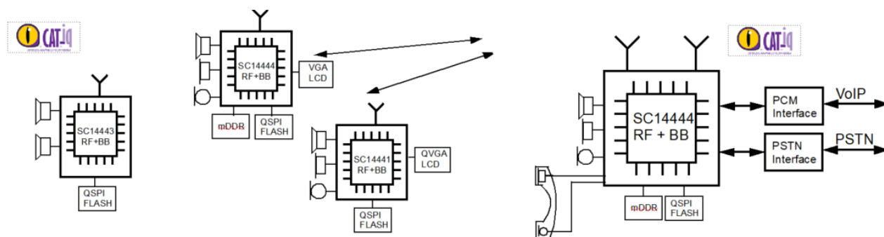
Figure 1. System diagram
