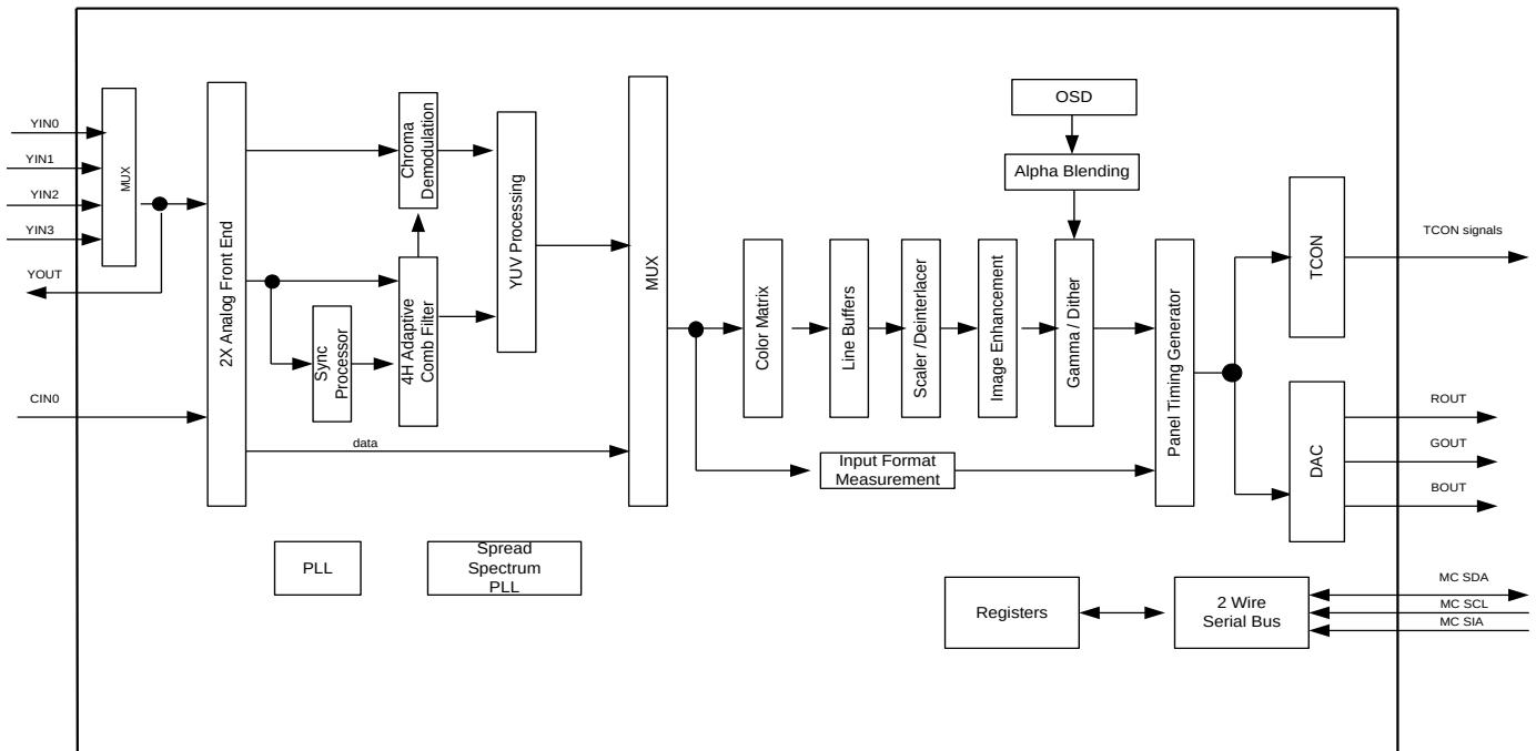
FIGURE 1. TW8807 FLAT PANEL TV/MONITOR CONTROLLER FUNCTIONAL BLOCK DIAGRAM
