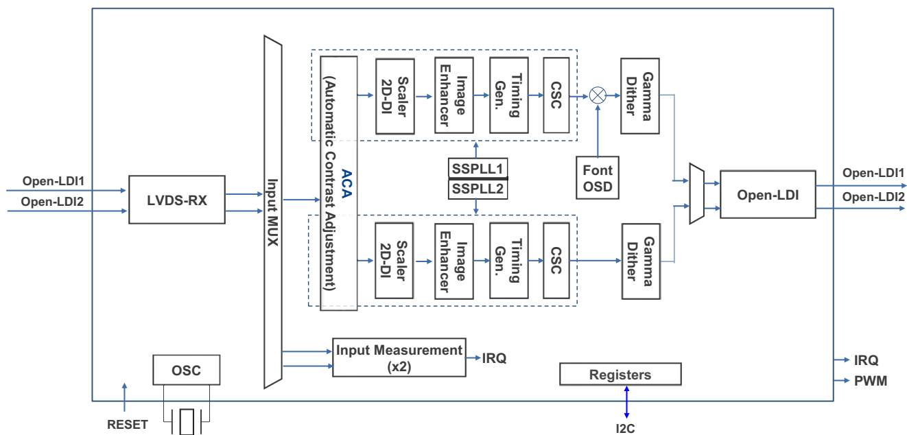
Figure 1. TW8849 Functional Block Diagram
