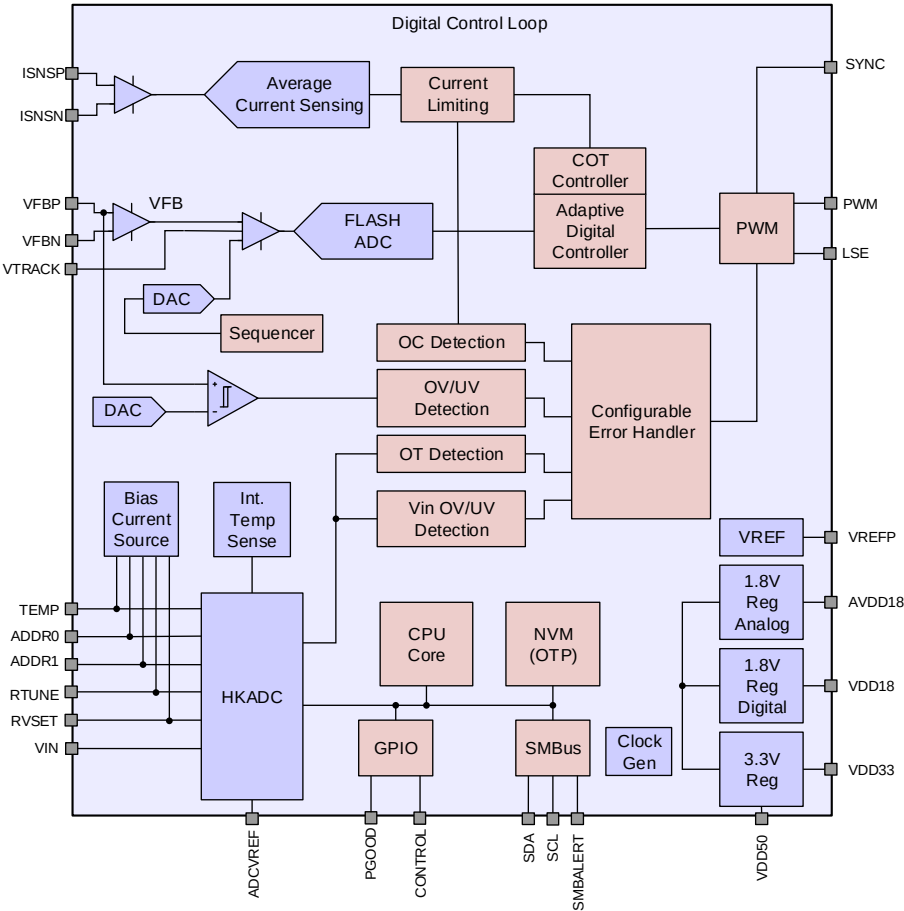
ZSPM1063 Block Diagram
