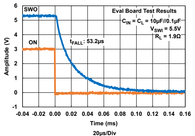
Figure 29. Turn-Off Waveform, 5.5V, C_L = 10.1\mu\text{F} (Characterization Results)
