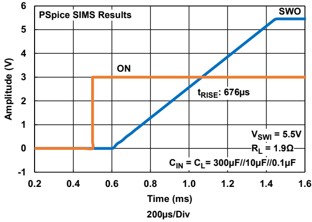
Figure 18. Turn-On Waveform, 5.5V, C_L = 310.5\mu F (PSpice Results)
