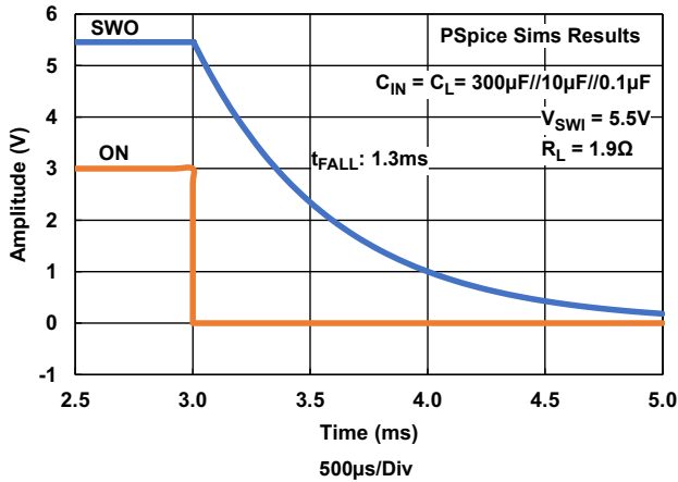
Figure 20. Turn-Off Waveform, 5.5V, C_L = 310.5\mu F (PSpice Results)
