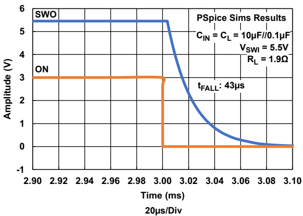
Figure 28. Turn-Off Waveform, 5.5V, C_L = 10.1\mu\text{F} (PSpice Results)
