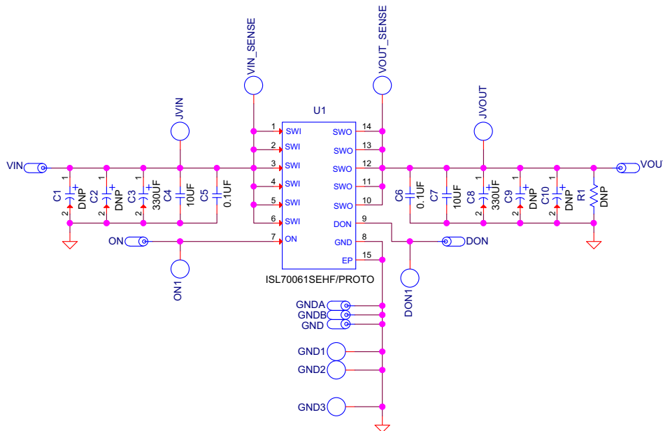
Figure 5. ISL70061SEHEV1Z Rev. A Evaluation Board Schematic
