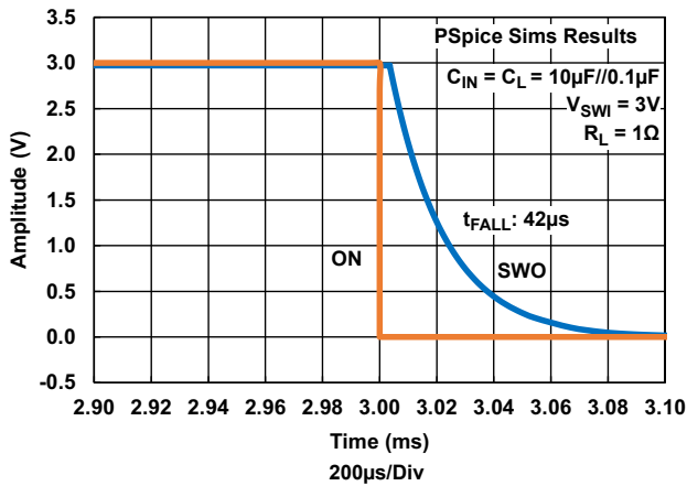
Figure 24. Turn-Off Waveform, 3V, C_L = 10.1\mu\text{F} (PSpice Results)
