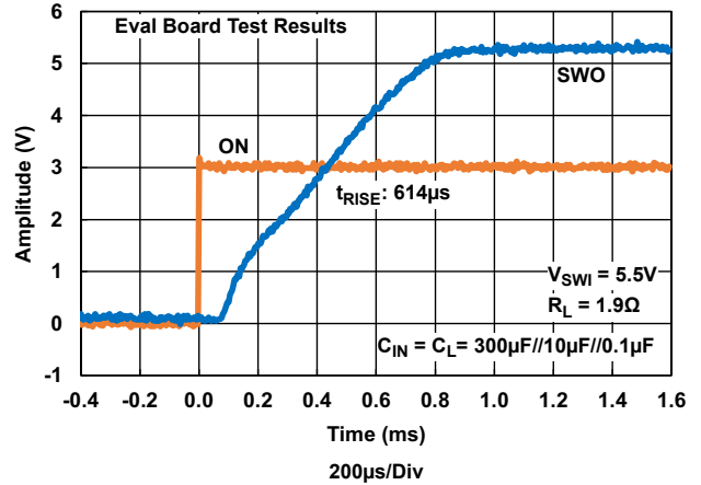
Figure 19. Turn-On Waveform, 5.5V, C_L = 310.5\mu F (Characterization Results)
