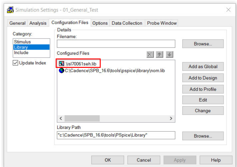
Figure 2. ISL70061SEH.LIB
