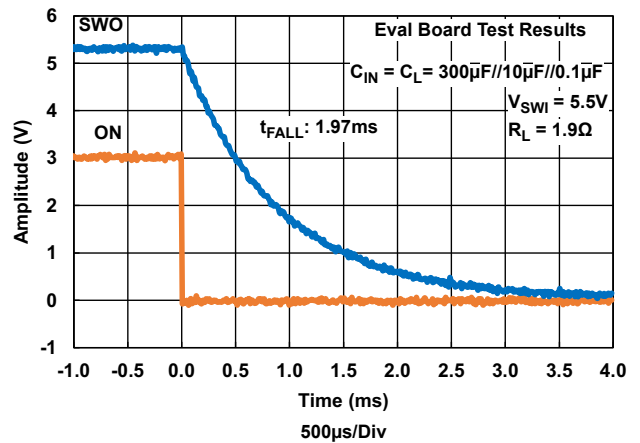
Figure 21. Turn-Off Waveform, 5.5V, C_L = 310.5\mu F (Characterization Results)
