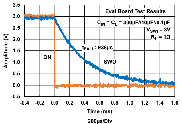
Figure 17. Turn-Off Waveform, 3V, C_L = 310.5\mu\text{F} (Characterization Results)
