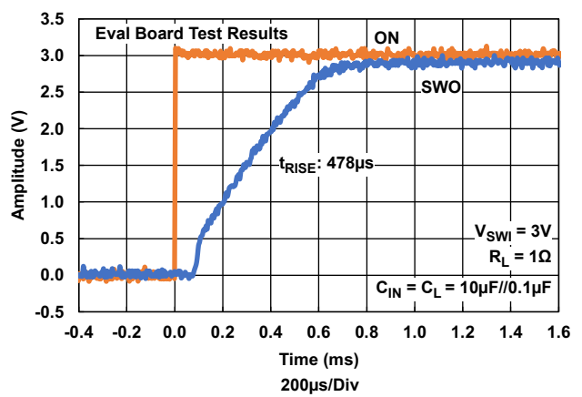
Figure 23. Turn-On Waveform, 3V, C_L = 10.1\mu F (Characterization Results)
