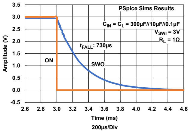
Figure 16. Turn-Off Waveform, 3V, C_L = 310.5\mu\text{F} (PSpice Results)
