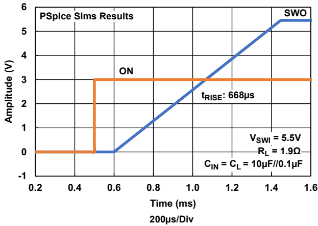
Figure 26. Turn-On Waveform, 5.5V, C_L = 10.1\mu\text{F} (PSpice Results)
