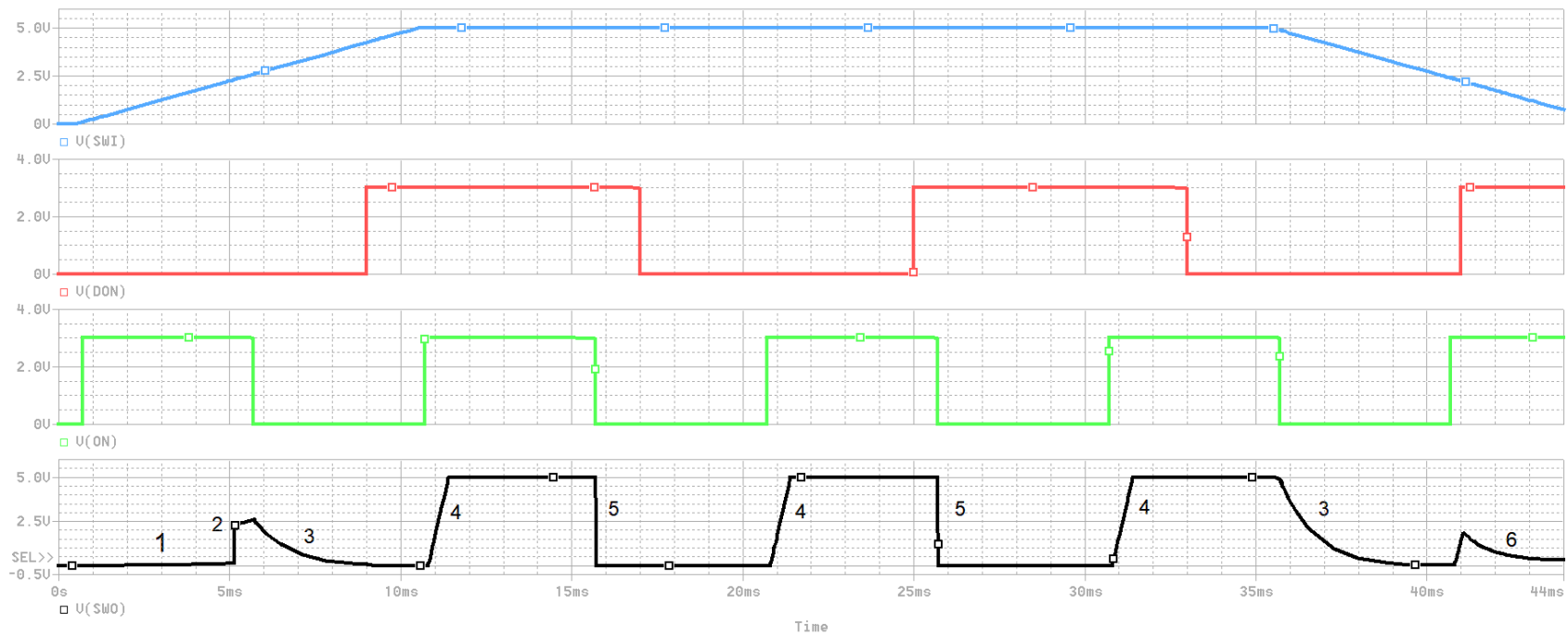
Figure 4. ISL70061SEH PSpice General Functional Simulation Results
