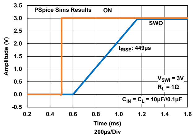
Figure 22. Turn-On Waveform, 3V, C_L = 10.1\mu F (PSpice Results)
