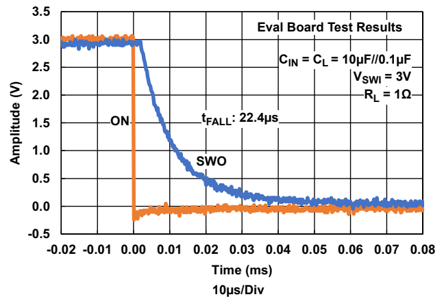
Figure 25. Turn-Off Waveform, 3V, C_L = 10.1\mu\text{F} (Characterization Results)
