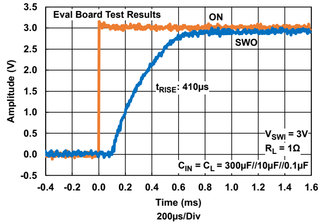
Figure 15. Turn-On Waveform, 3V, C_L = 310.5\mu\text{F} (Characterization Results)
