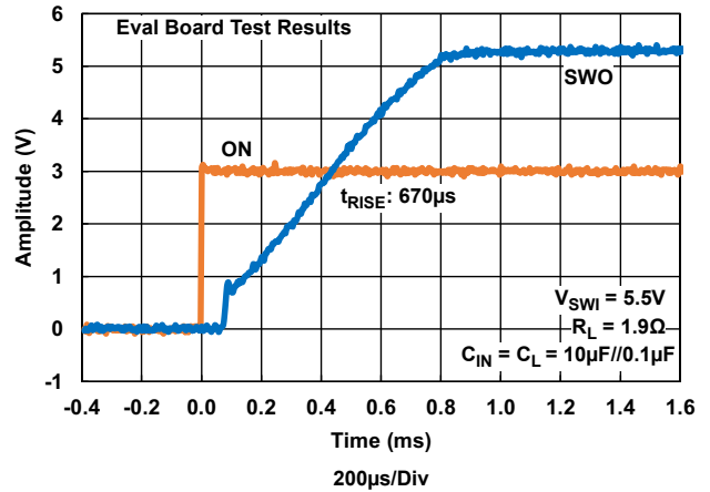
Figure 27. Turn-On Waveform, 5.5V, C_L = 10.1\mu\text{F} (Characterization Results)
