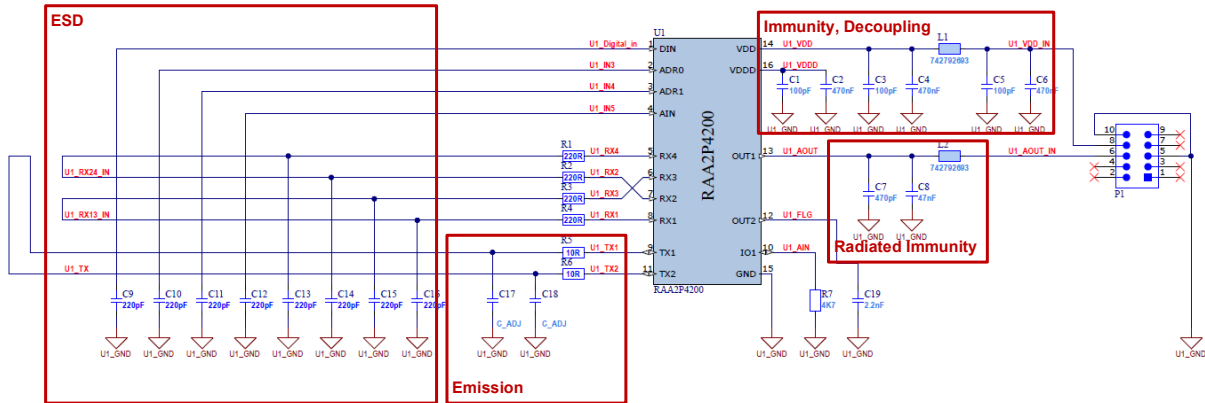
Figure 1. EMC Schematic
