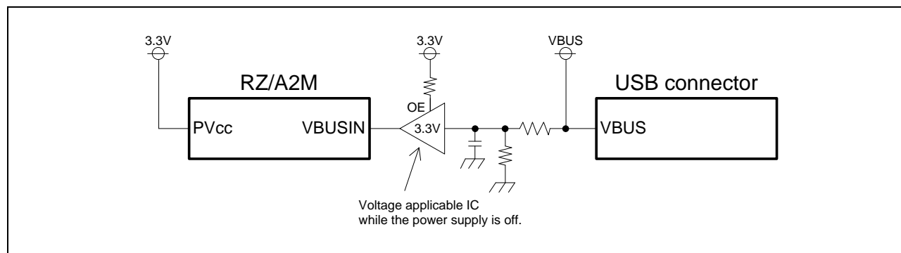
Figure 5 VBUSIN Circuit Example
