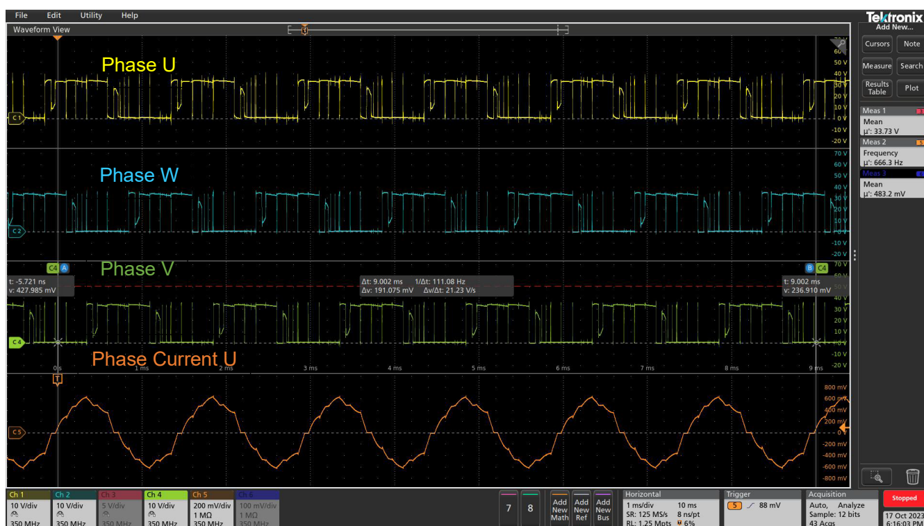
Figure 8: 150-degree Commutation
