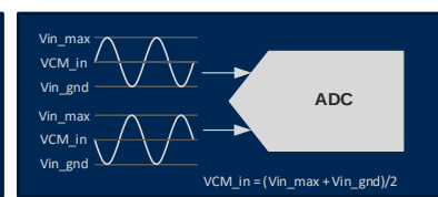
Fig.15c: Fully-Differential
