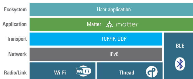
Figure 2: Matter architecture
