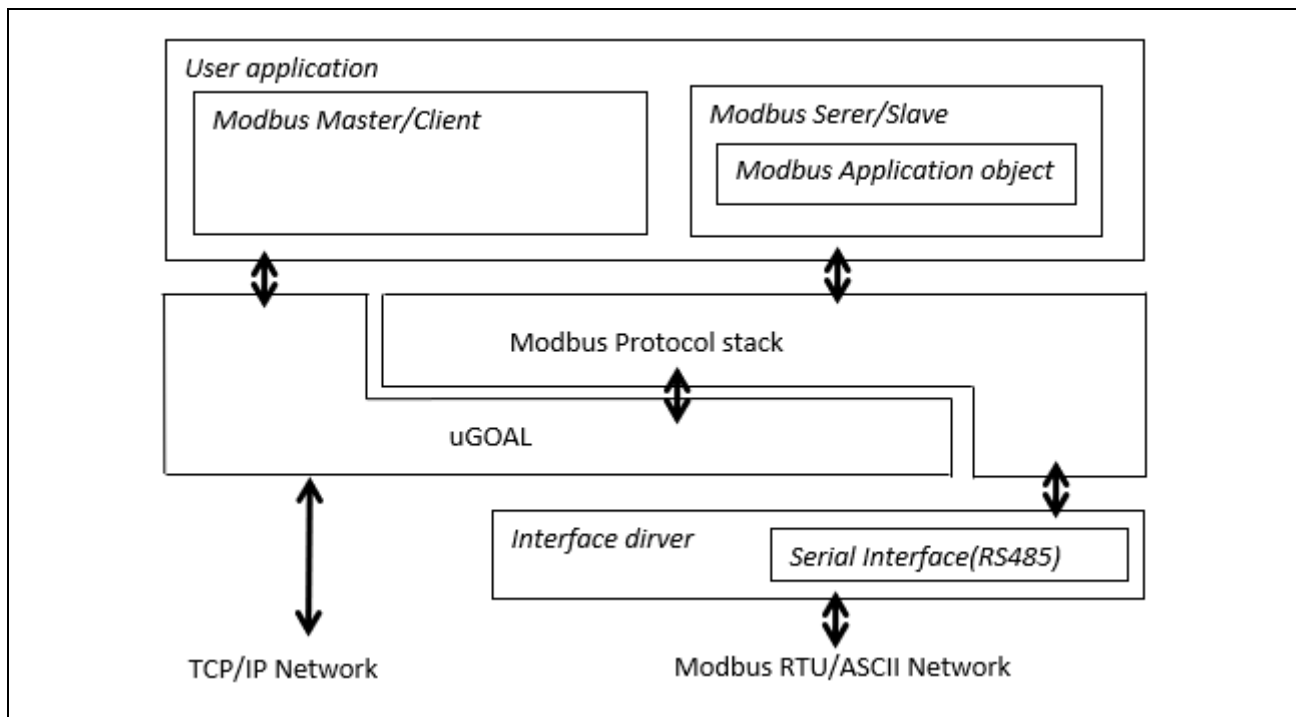
Figure 1-1 System Structure
