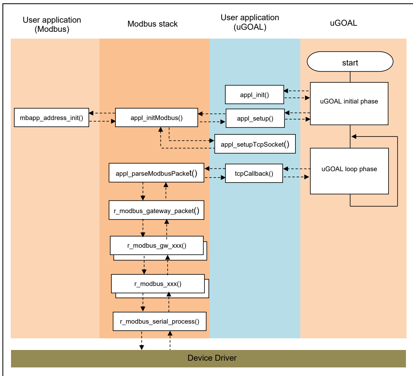
Figure 2-4 Modbus TCP Gateway program flow
